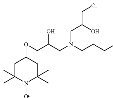
4-{3-[Butyl-(3-chloro-2-hydroxy-propyl)-amino]-2-hydroxy-propoxy}-2,2,6,6-tetramethyl-piperidin-1-oxyl
