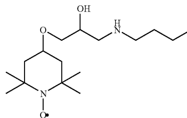
4-(3-Butylamino-2-hydroxy-propoxy)-2,2,6,6-tetramethyl-piperidin-1-oxyl
