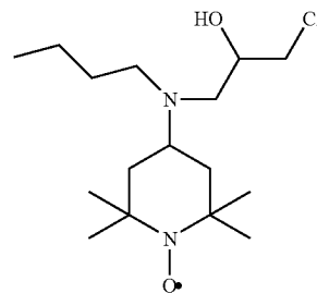
N-Butyl-N-(2-hydroxy-3-chloro)propyl-1-oxyl-2,2, 6,6-tetramethyl-4-aminopiperidine
