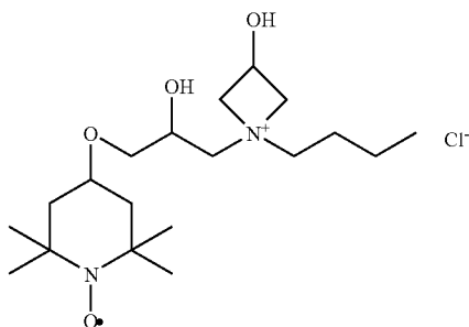
1-Butyl-3-hydroxy-1-[2-hydroxy-3-(1-oxyl-2,2,6,6-tetramethyl-piperidin-4-yloxy)-propyl]-azetidininium chloride
