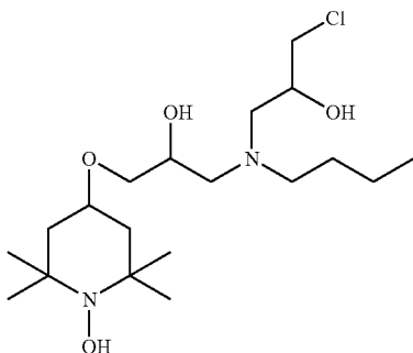
4-{3-[Butyl-(3-chloro-2-hydroxy-propyl)-amino]-2-hydroxy-propoxy}-2,2,6,6-tetramethyl-piperidin-1-ol
