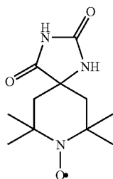
8-Oxyl-7,7,9,9-tetramethyl-1,3,8-triaza-spiro[4.5] decane-2,4-dione
