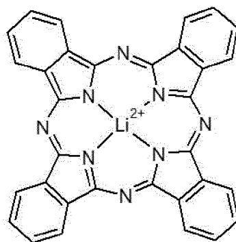
[Chemical Formula IV]
