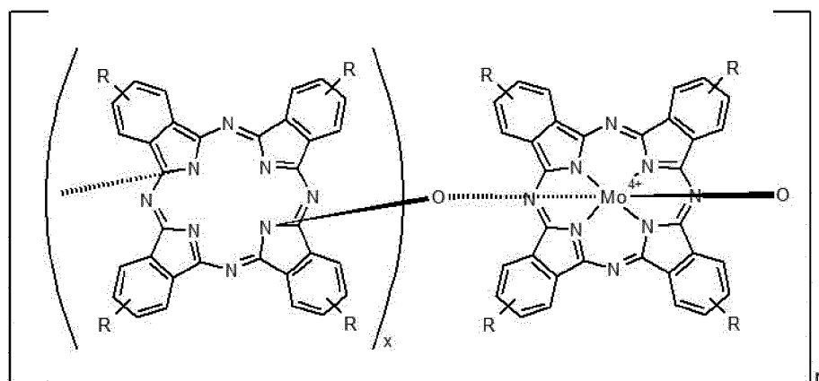
[Chemical Formula I]
