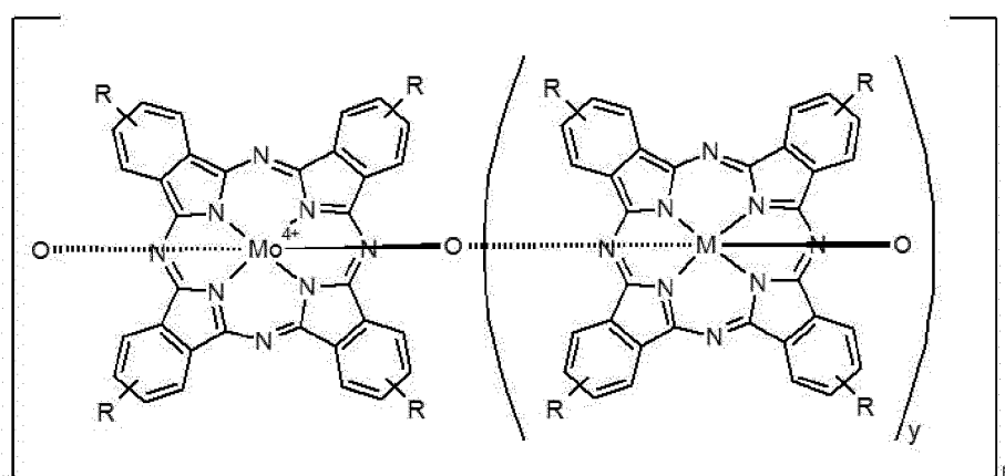
[Chemical Formula II]
