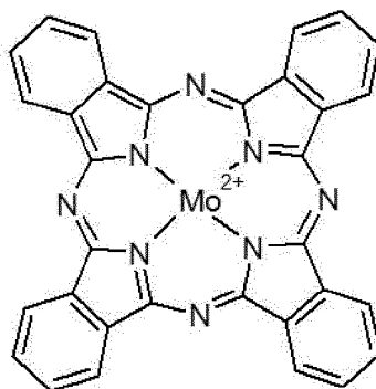
[Chemical Formula V]
