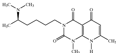
(R)-1,7-Dimethyl-3-(5-(N,N-dimethylamino)hexyl)pyrido[2,3-d]pyrimidine-2,4,5(1H,3H,8H)-trione, Acetic Acid Salt (CT-30271)
