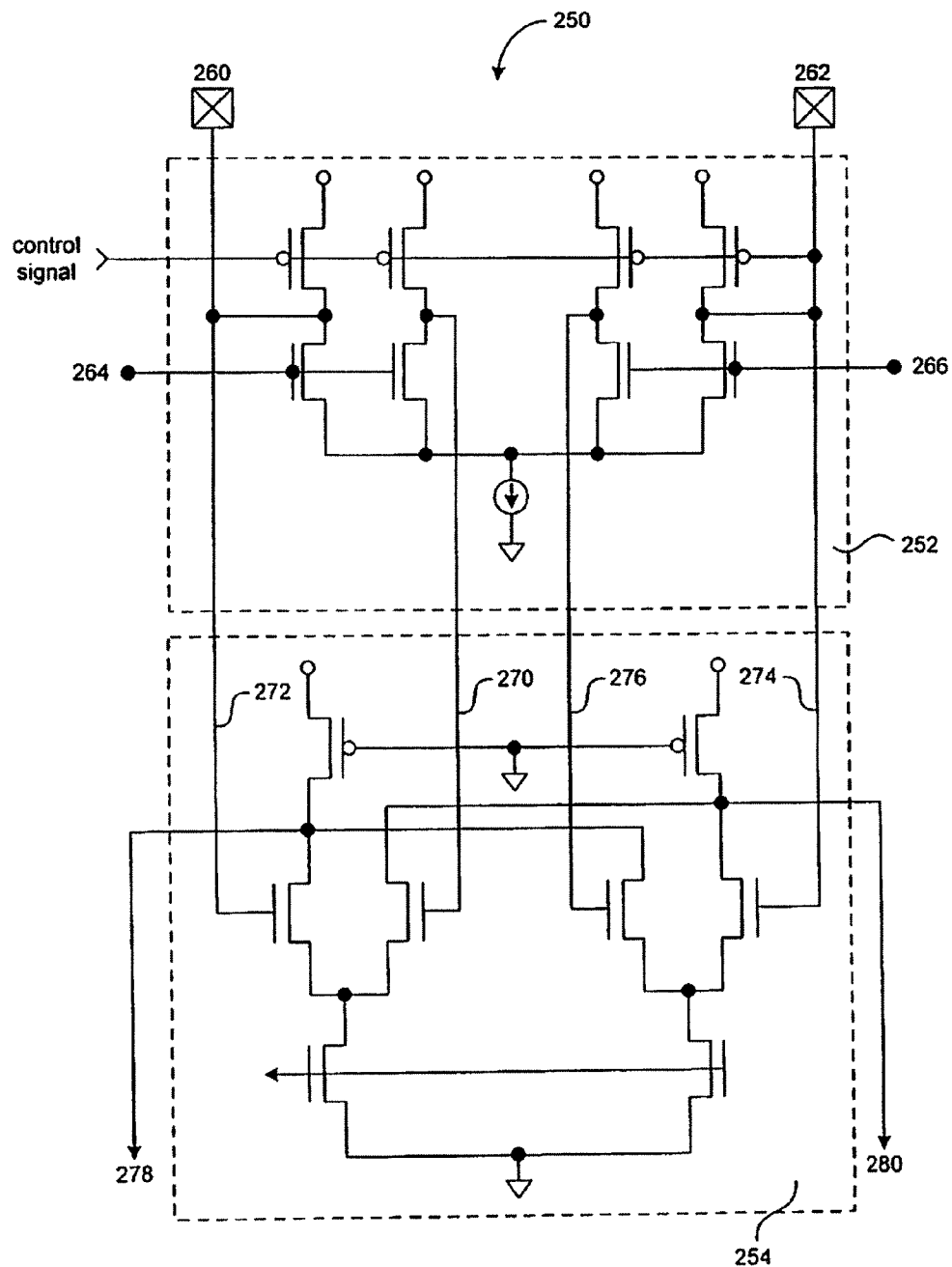
FIG. 2 (Prior Art)
