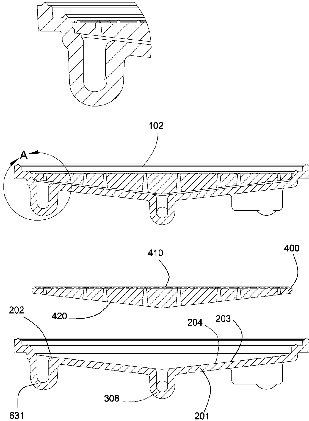
Detail A
