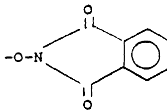
Oxypthalimide
