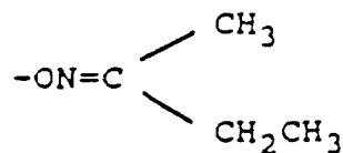
Methylethyl Ketoxime
