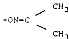
Acetone Oxime
