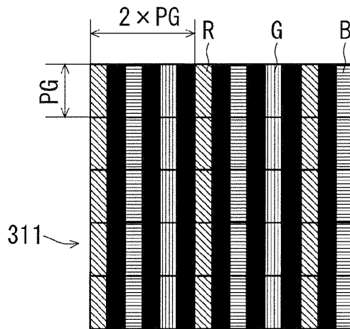
VERTICAL STRIPE ARRANGEMENT OF OPENING
