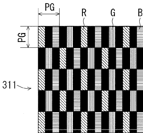
CHECKERED FLAG PATTERN ARRANGEMENT OF OPENING
