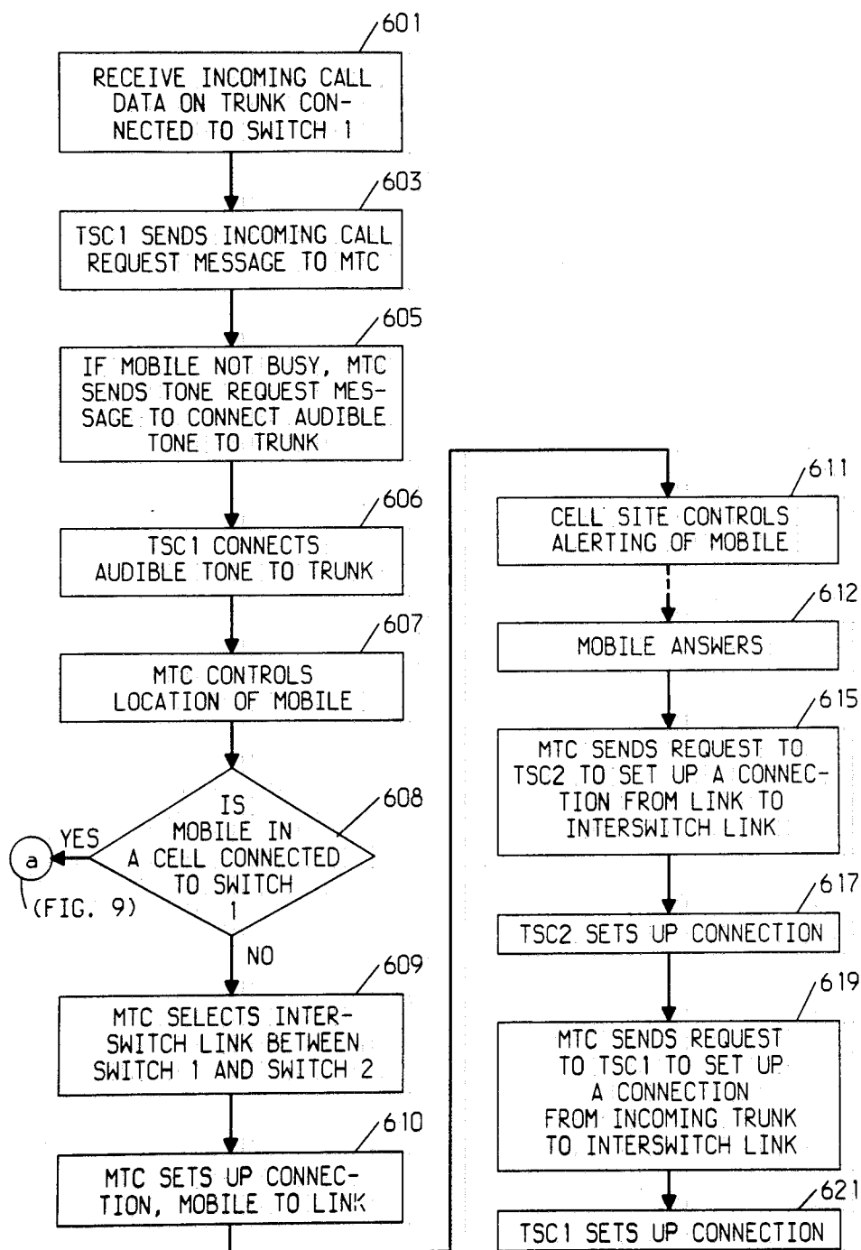
FIG. 15 INCOMING CALL: MULTISWITCH CONFIGURATION
