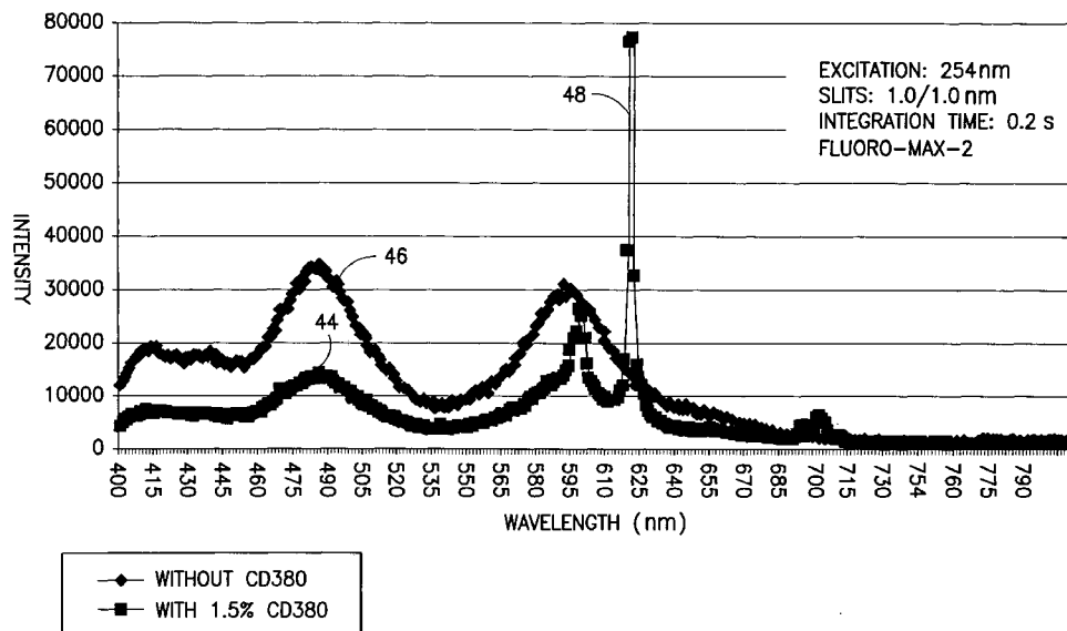
EMISSION SPECTRA OF HETEROGENEOUS BLACK FLUORESCENT INKS
