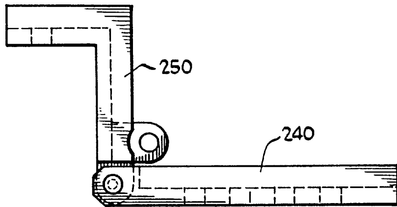
VERTICAL MOUNTING POSITION
