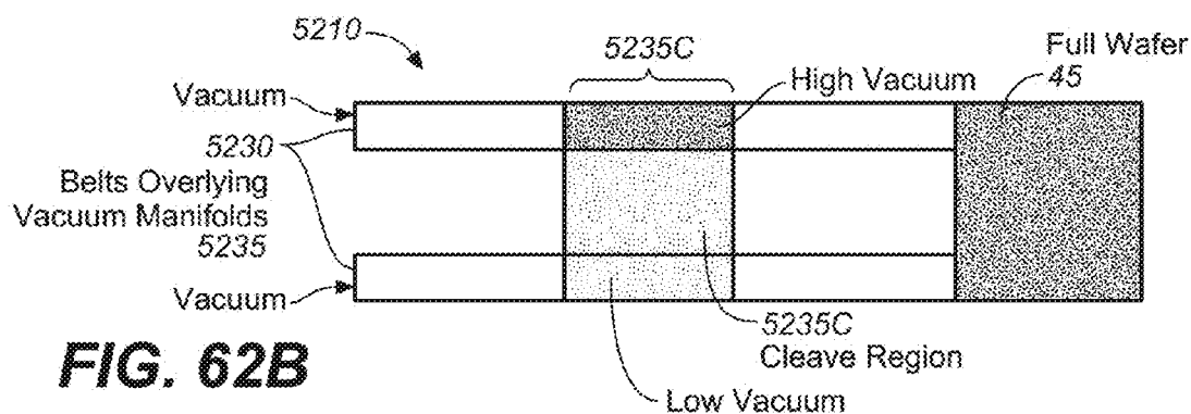
Top View of Cleave Tool
