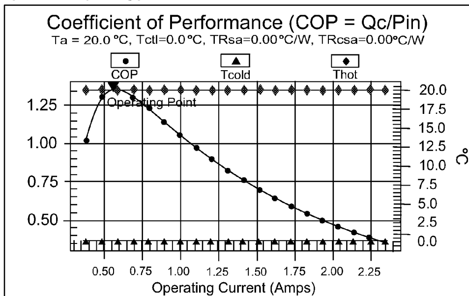
Optimum TE operating point at DT 20
