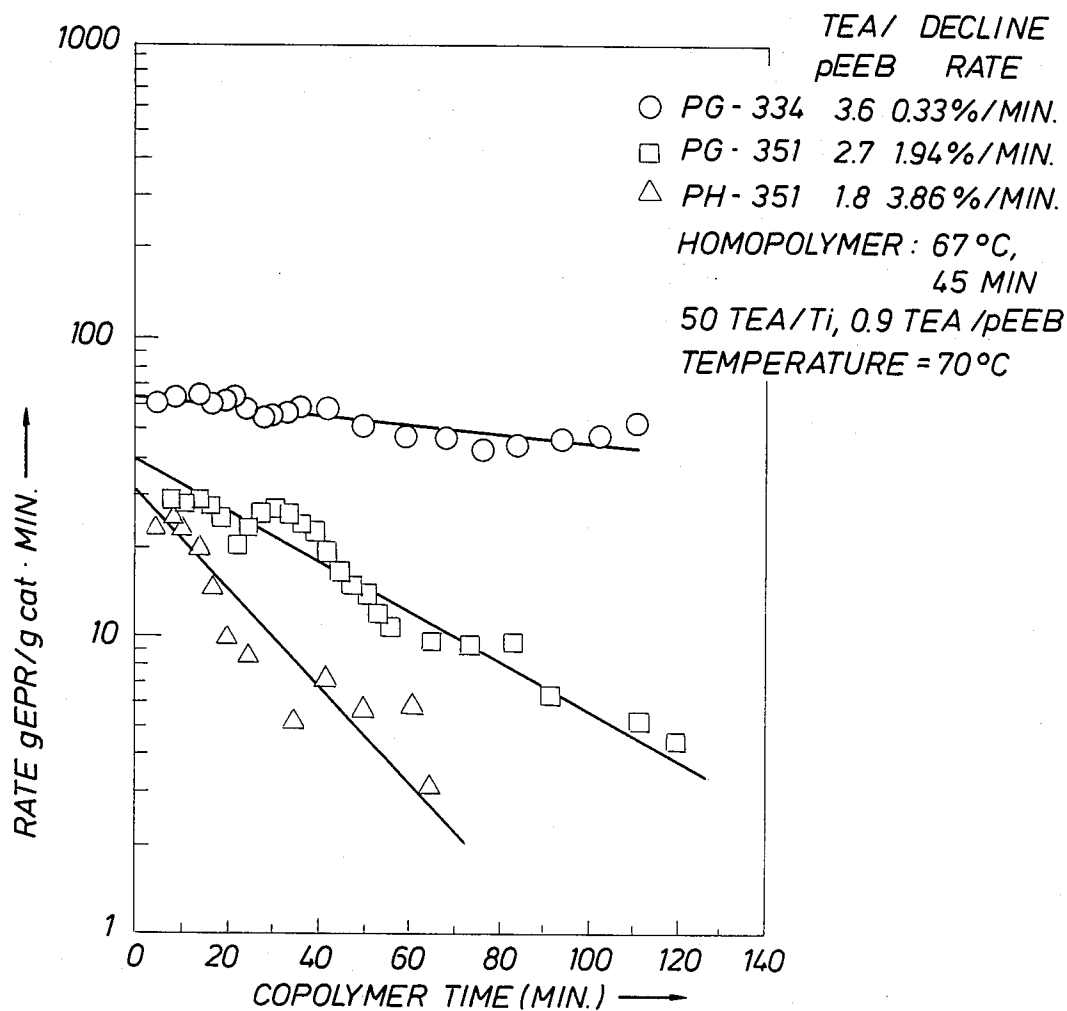
FIG. 1 EFFECT OF TEA/pEEB ON COPOLYMER DEACTIVATION RATE
