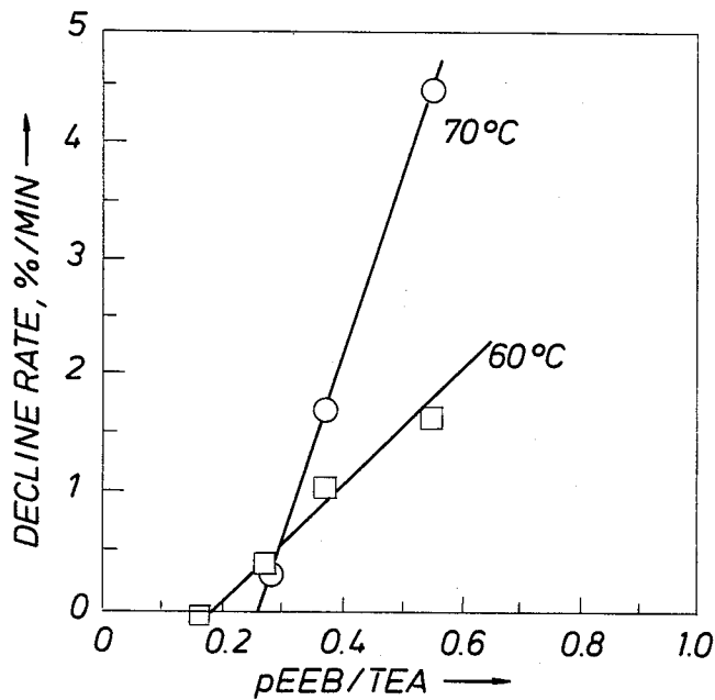
FIG. 2 COPOLYMER DEACTIVATION AS A FUNCTION OF TEA/pEEB
