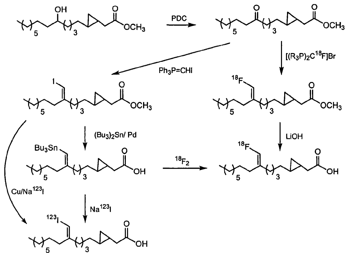
Synthesis of Exo- [ 18 F]Fluoro- or [ 123 I]iodo-3,4-Cyclopropylheptadecanoic Acid
