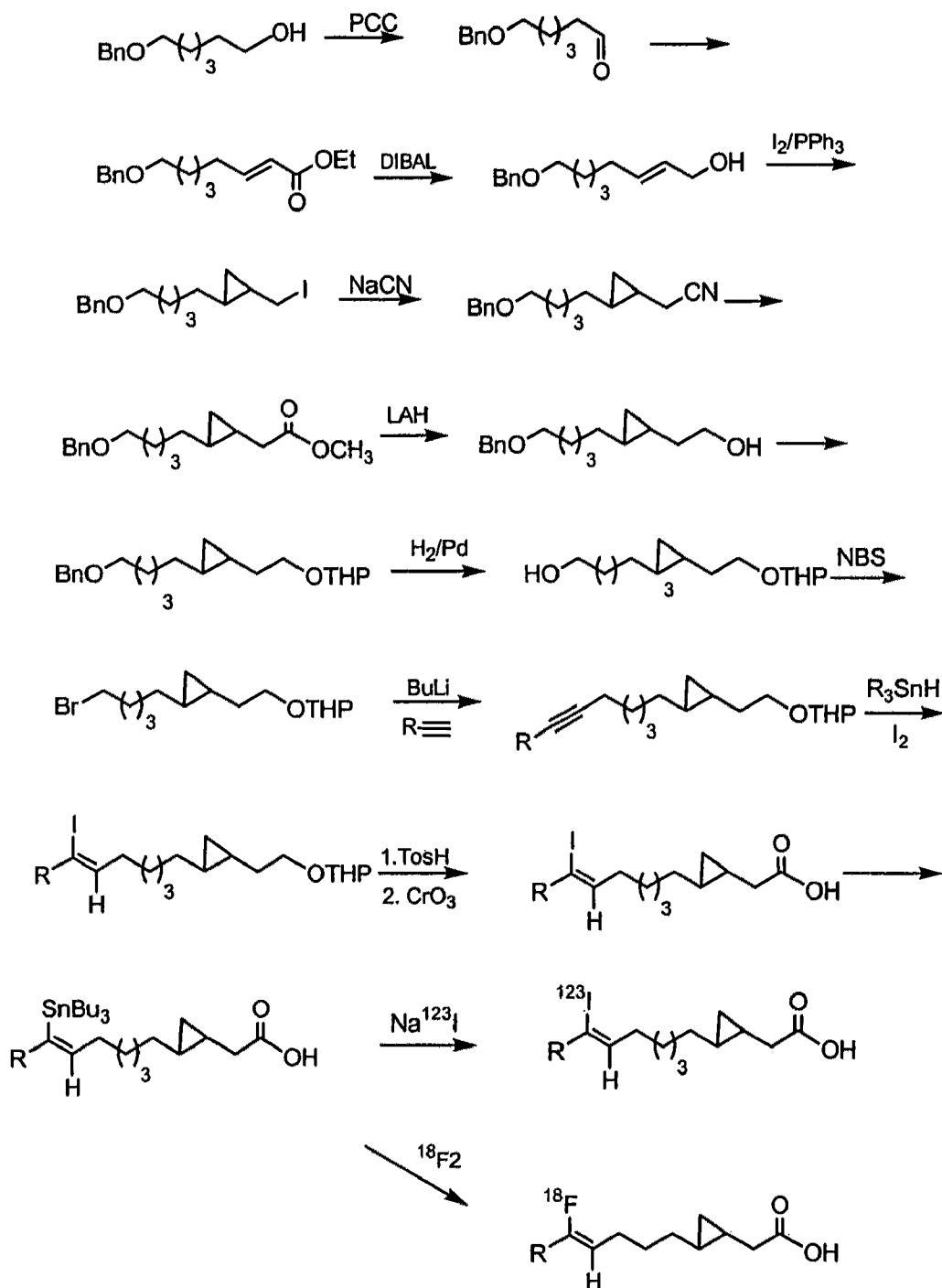
Synthesis of Endo- [ 18 F]Fluoro- or [ 123 I]iodo-3,4-Cyclopropylheptadecanoic Acid
