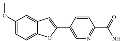
5-(5-methoxy-1-benzofuran-2-yl)pyridine-2-carboxamide
