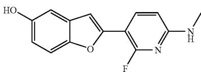
2-(2-fluoro-6-methylamino-pyridin-3-yl)-benzofuran-5-ol
