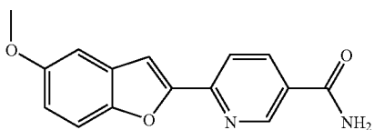
6-(5-methoxy-1-benzofuran-2-yl)nicotinamide
