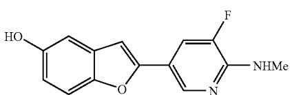
2-(5-fluoro-6-methylamino-pyridin-3-yl)-benzofuran-5-ol
