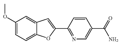
6-(5-methoxy-1-benzofuran-2-yl)nicotinamide
