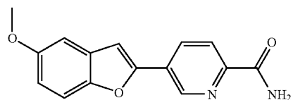
5-(5-methoxy-1-benzofuran-2-yl)pyridine-2-carboxamide
