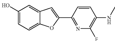
2-(6-fluoro-5-methylamino-pyridin-2-yl)-benzofuran-5-ol
