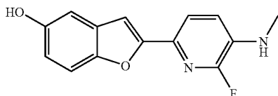
d) 2-(6-Fluoro-5-methylamino-pyridin-2-yl)-benzofuran-5-ol
