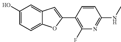
2-(2-Fluoro-6-methylamino-pyridin-3-yl)-benzofuran-5-ol
