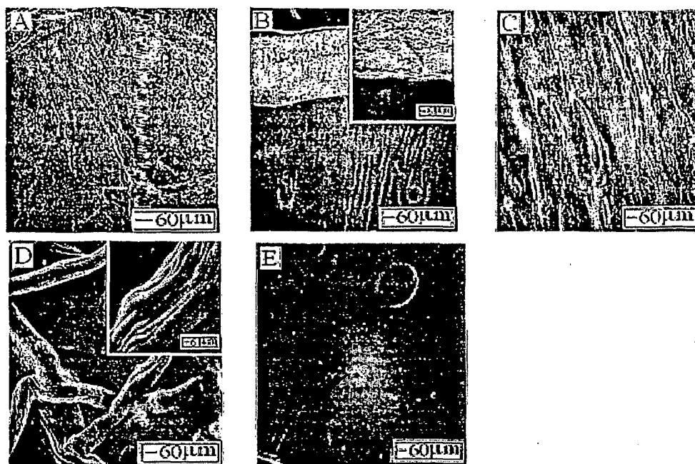
Figure 4. Scanning Electron Micrographs (SEM) of cellulose/poly-2-hydroxymethylmethacrylate (PHEMA). (A) cellulose/PHEMA 20/80; (B) cellulose/PHEMA 40/60; (C) cellulose/PHEMA 60/40(1); (D) cellulose/PHEMA 60/40(2); (E) cellulose/PHEMA 80/20 ( \times 500 and \times 5000 ).
