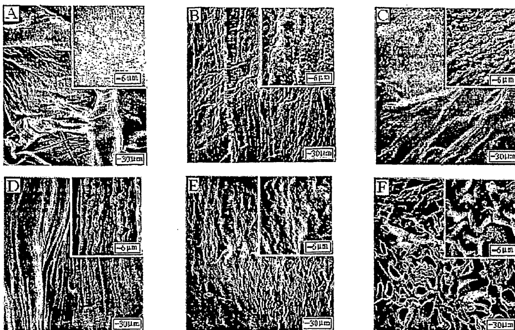
Figure 3. Scanning Electron Micrographs (SEM) of cellulose (wood pulp, DP=1056)/polyacrylonitrile (PAN) blend. (A) regenerated cellulose; (B) cellulose/PAN; 20/80 (weight ratio); (C) cellulose/PAN 40/60; (D) cellulose/PAN 60/40; (E) Cellulose/PAN, 80/20; (F) Regeneration PAN ( \times 500 and \times 5000 )
