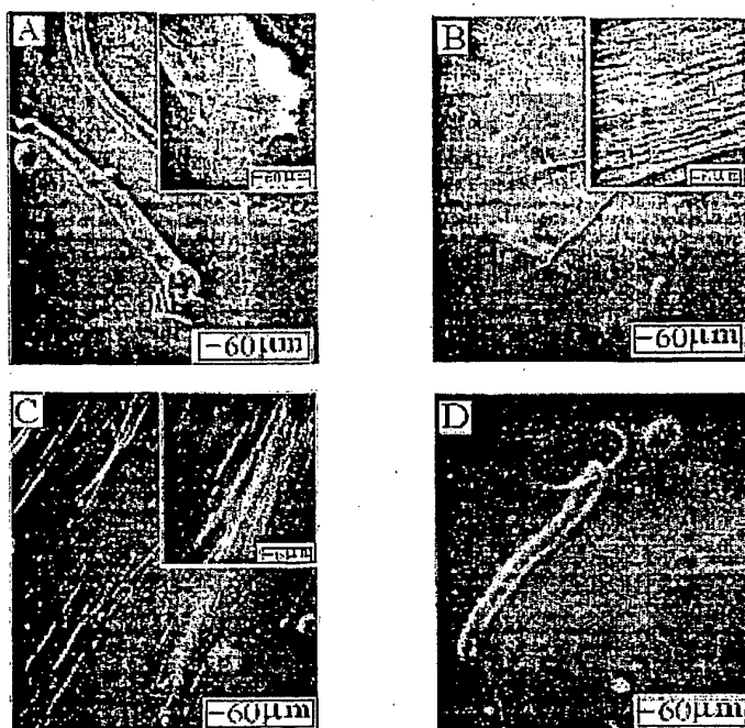
Figure 5. Scanning Electron Micrographs (SEM) of Cellulose/PVA blend at different ratio A: cellulose/PVA 20/80; B: cellulose/PVA 40/60; C: cellulose/PVA 60/40; D: cellulose/PVA 80/20. ( \times 500 and \times 5000 ). Equipment and procedure are similar to Figure 1.
