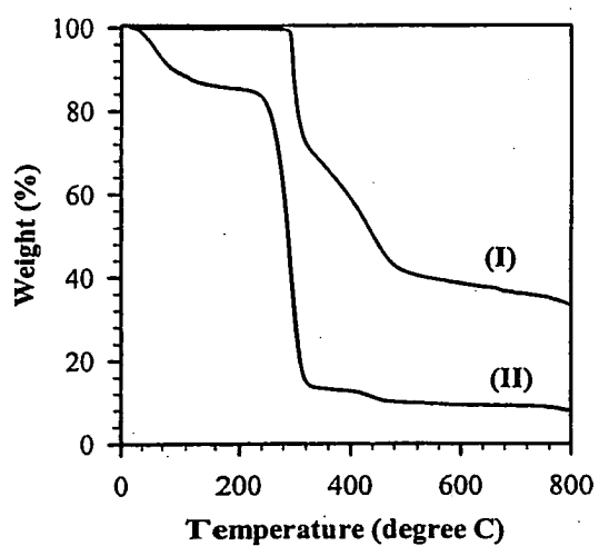
Figure 2. Thermogravimetric analysis (TGA) of (I) pure PAN and (II) regenerated PAN powder.
