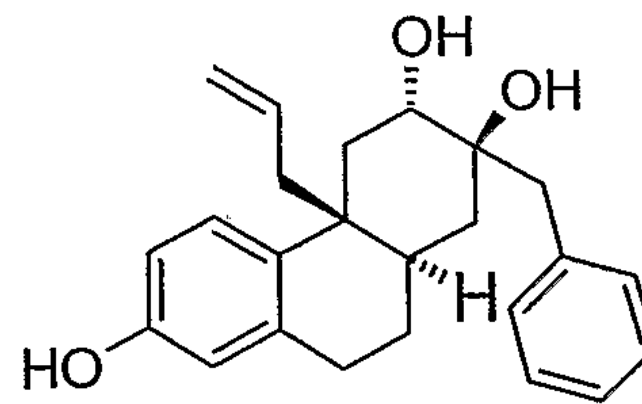
Example 24
