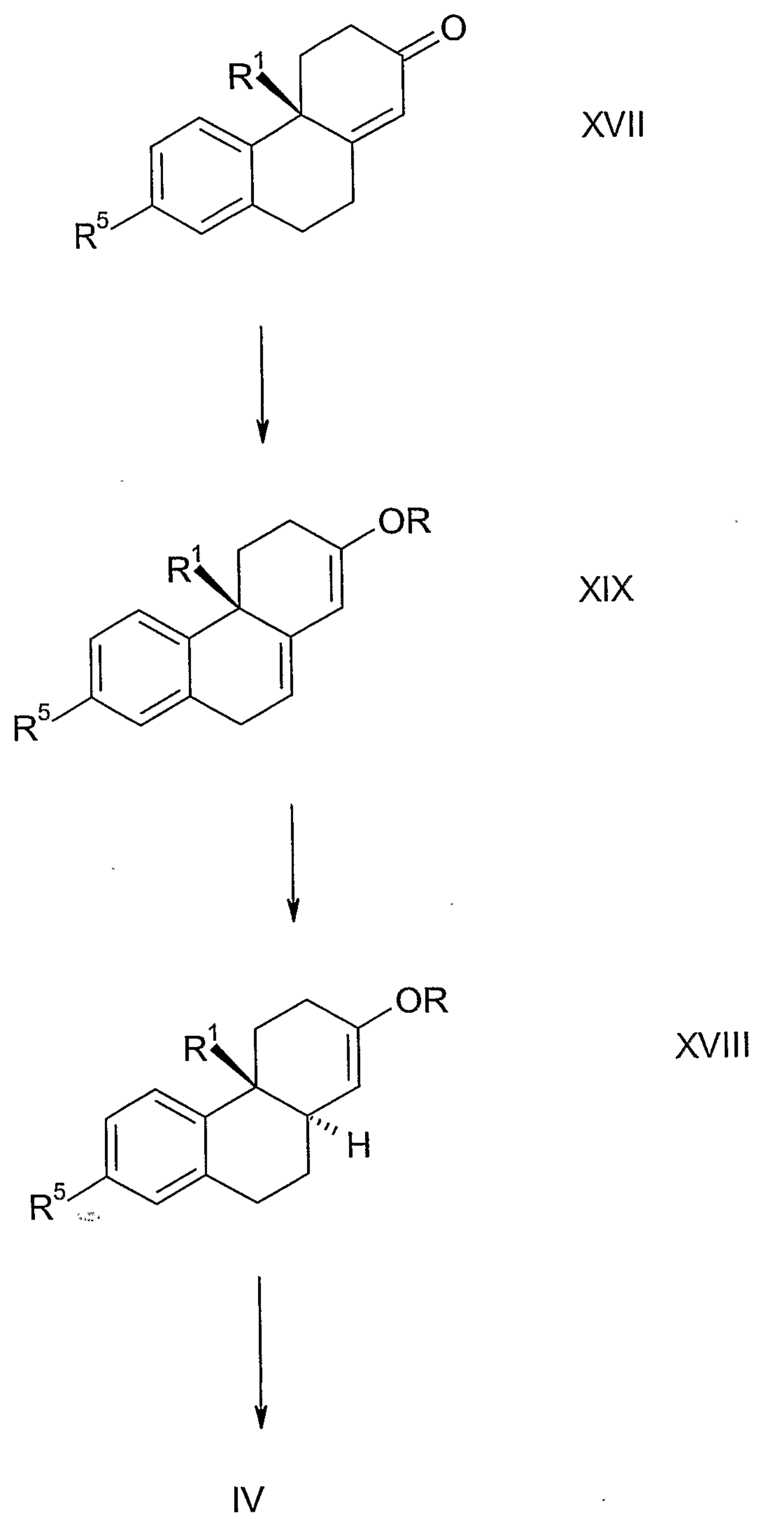
Scheme 7
