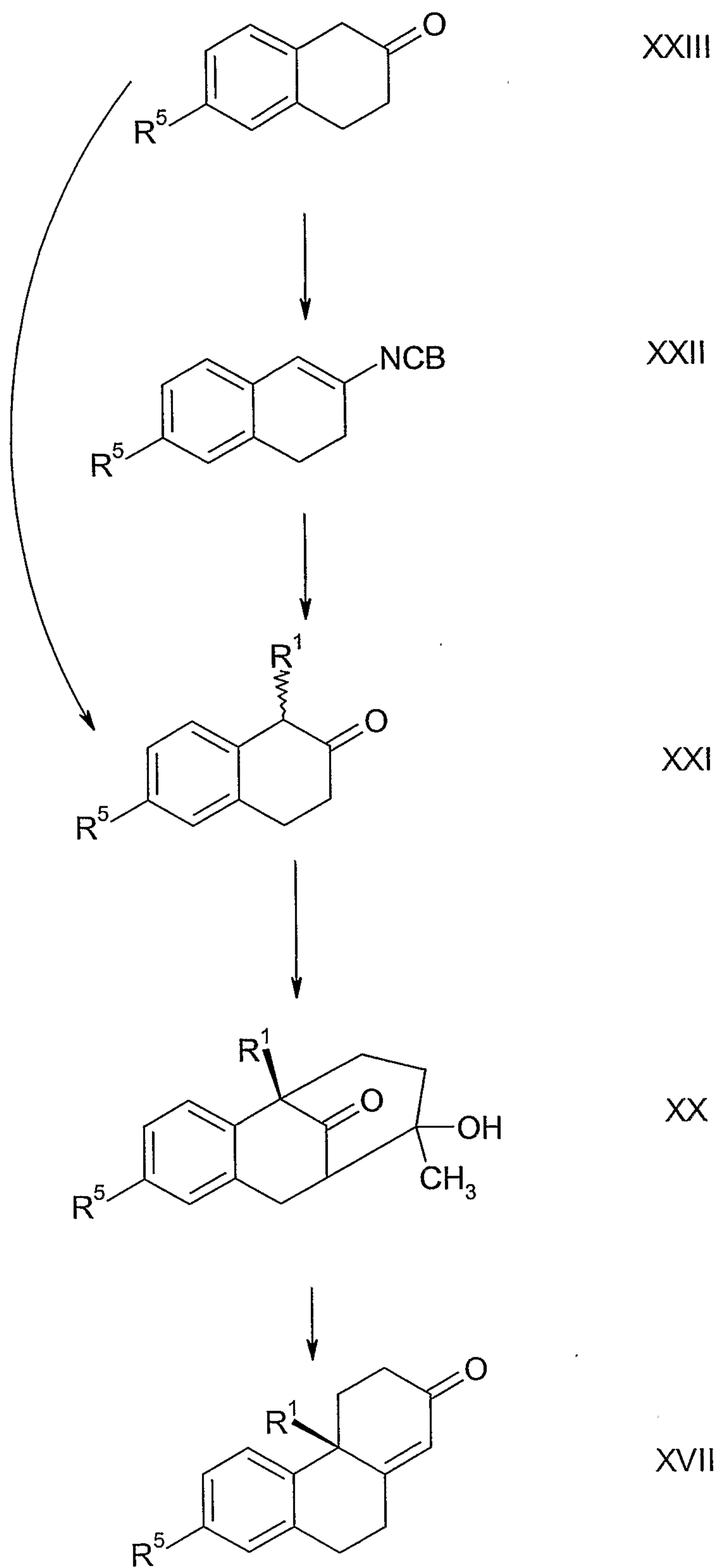
Scheme 8
