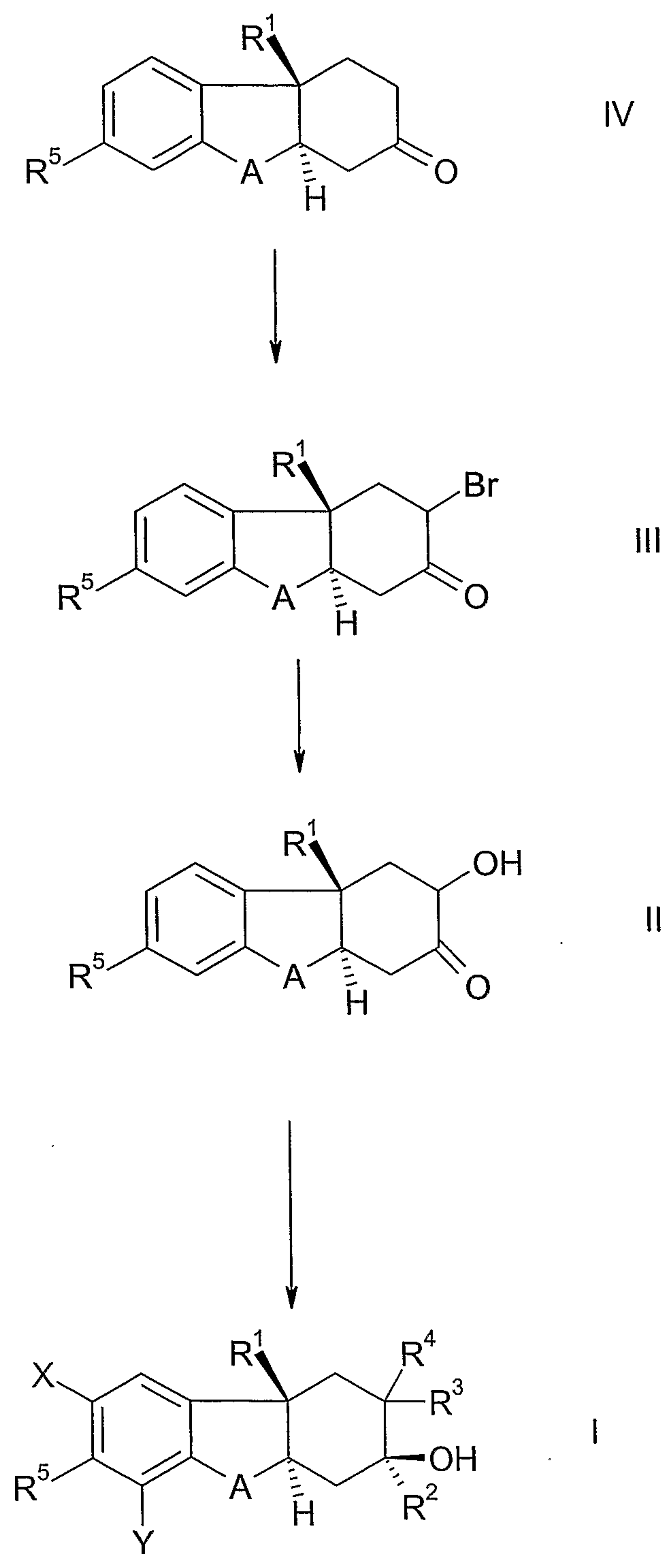
Scheme 1
