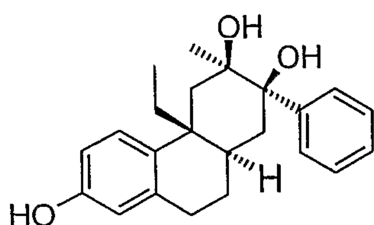
Example 42
