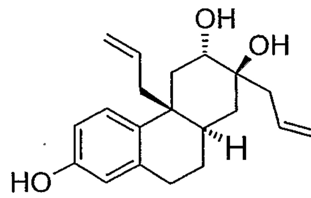
Example 26
