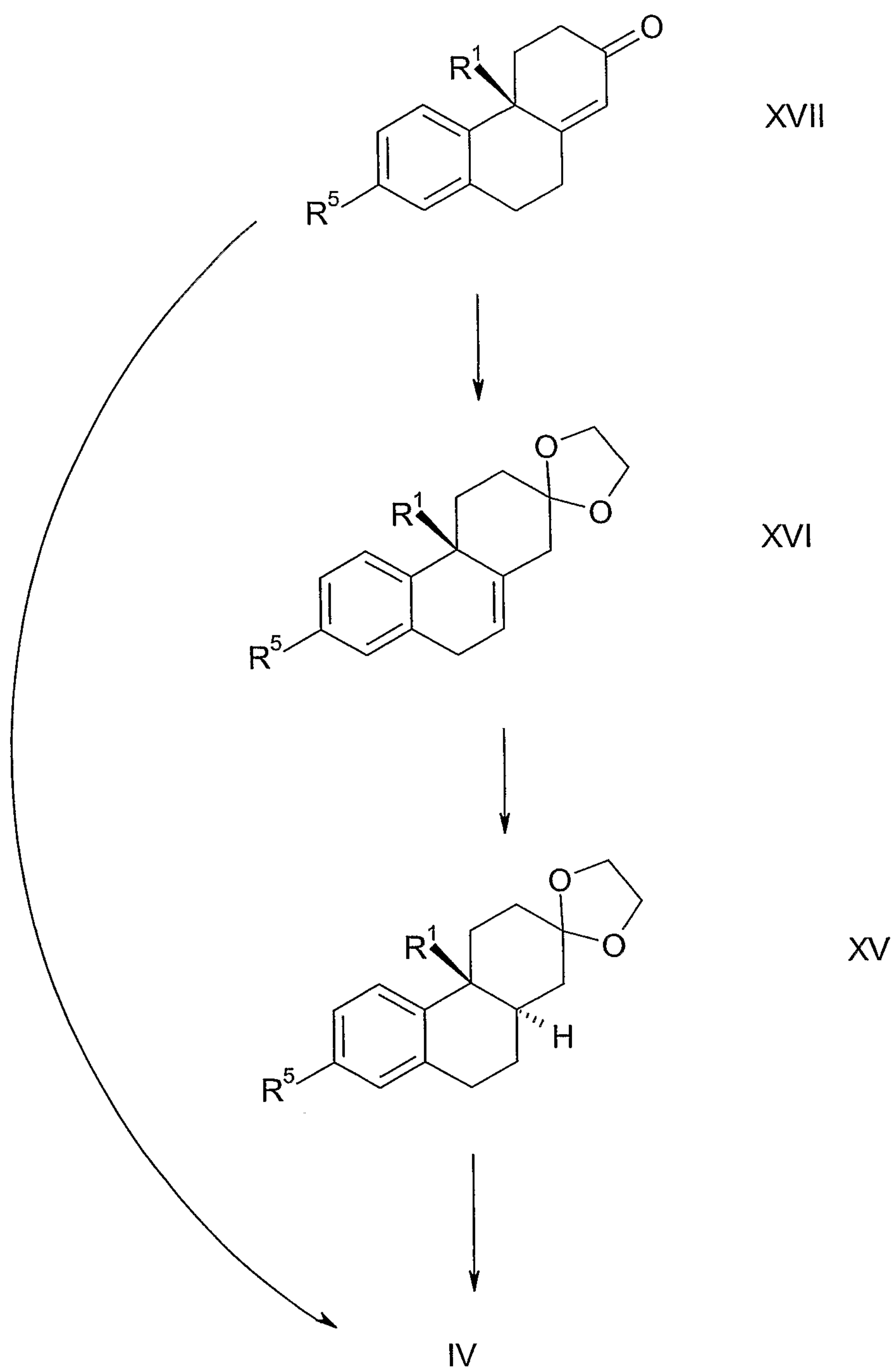
Scheme 6
