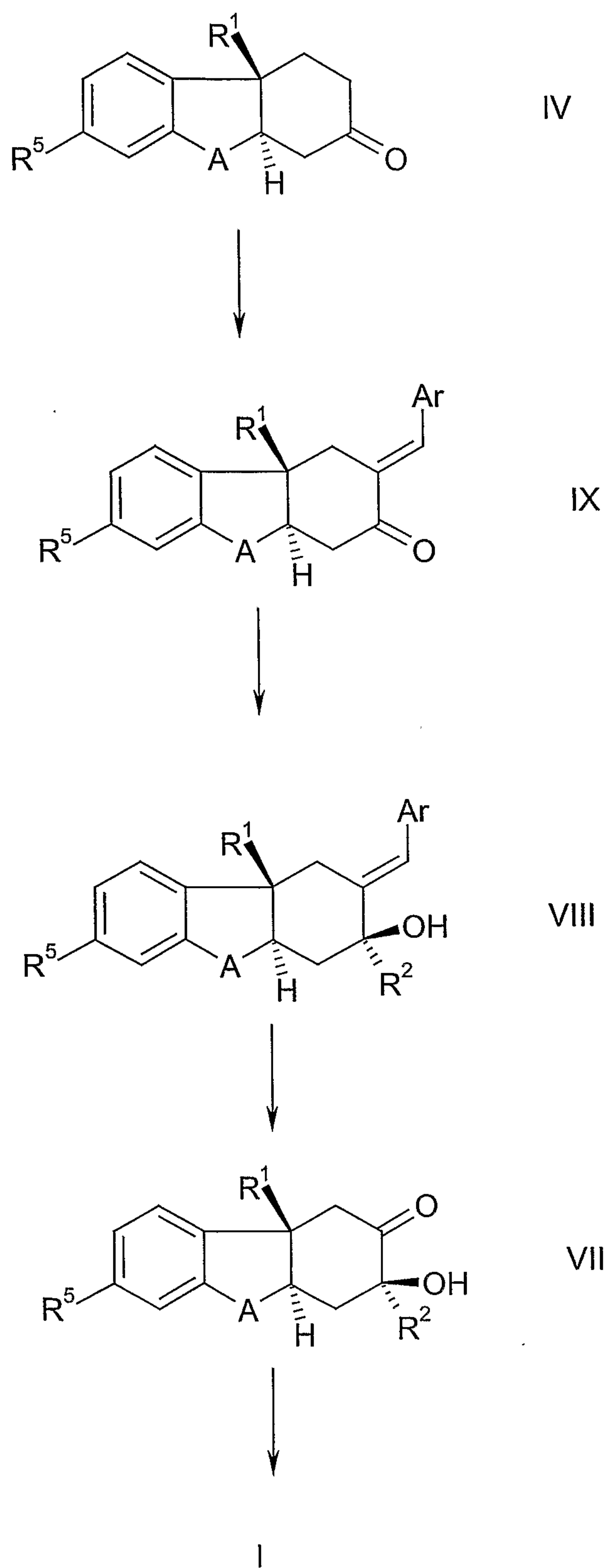
Scheme 3
