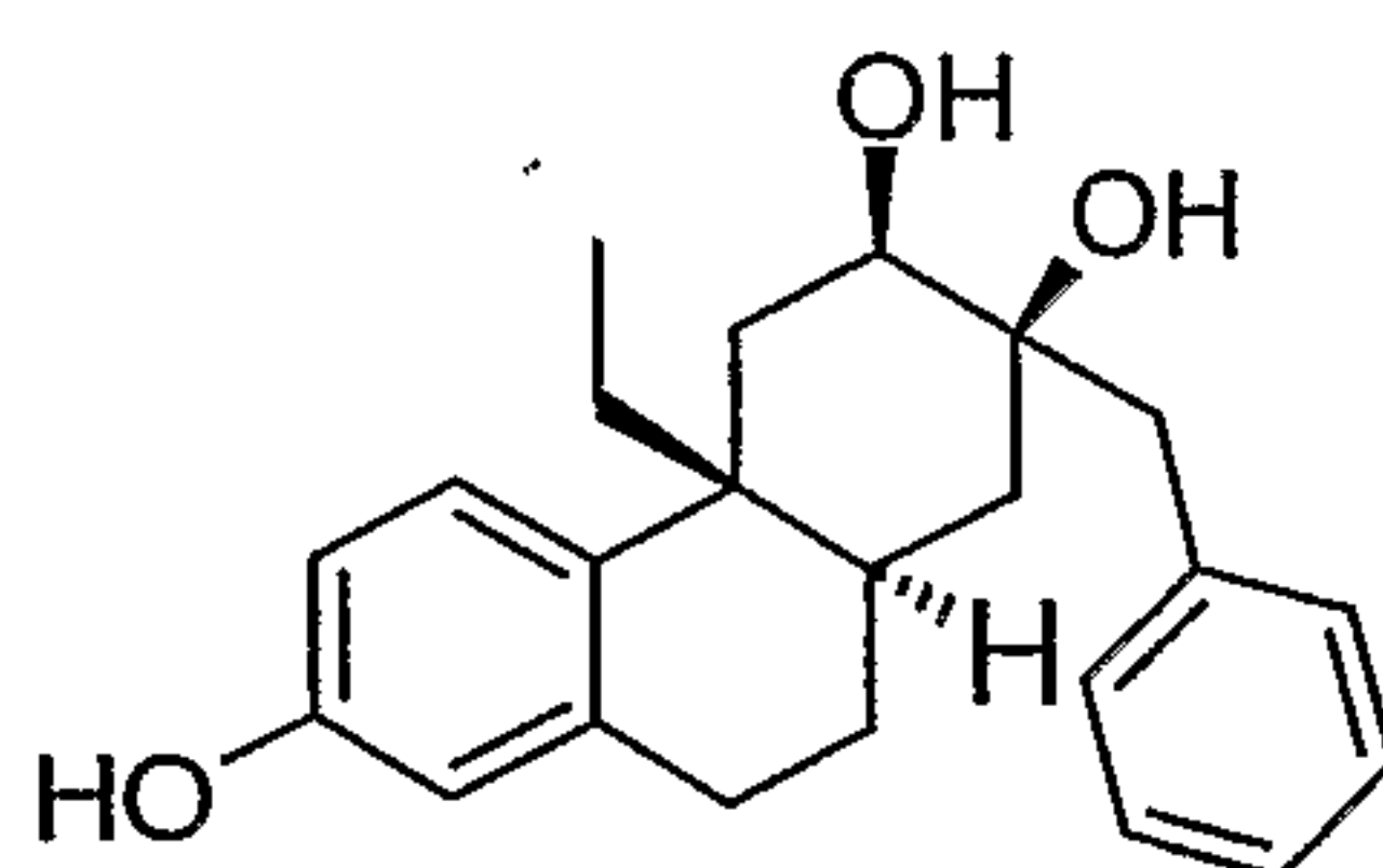
Example 21
