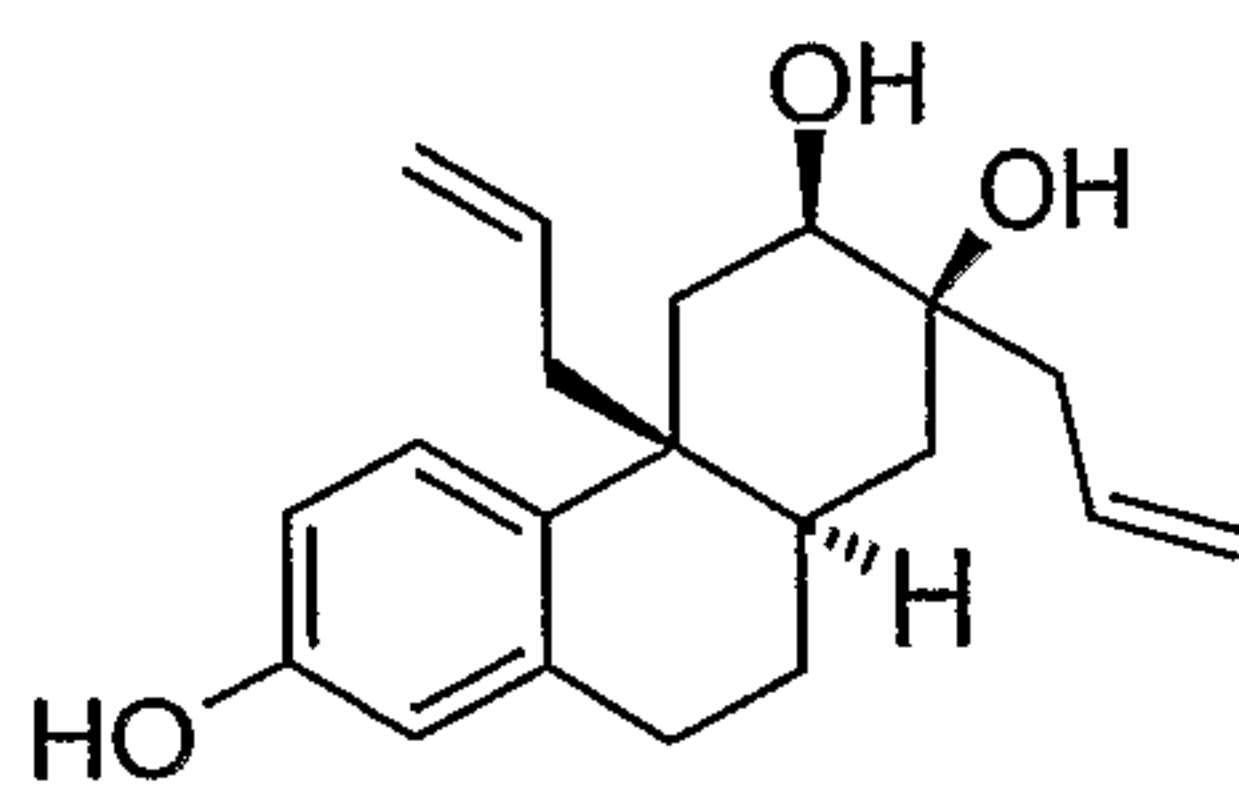
Example 25
