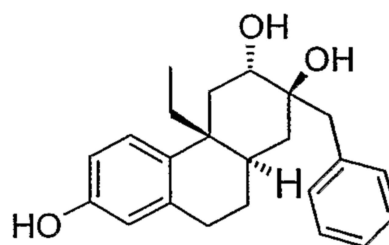
Example 22
