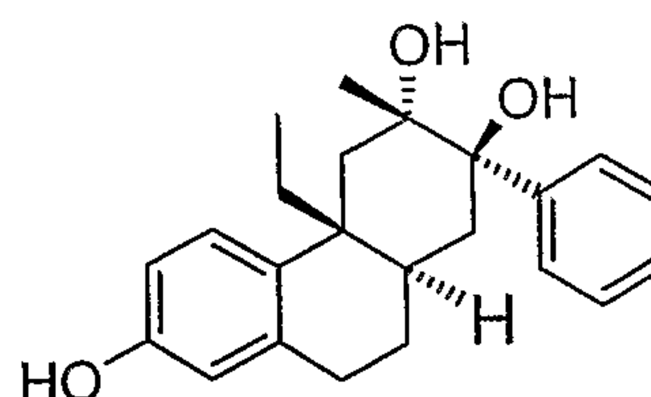
Example 43
