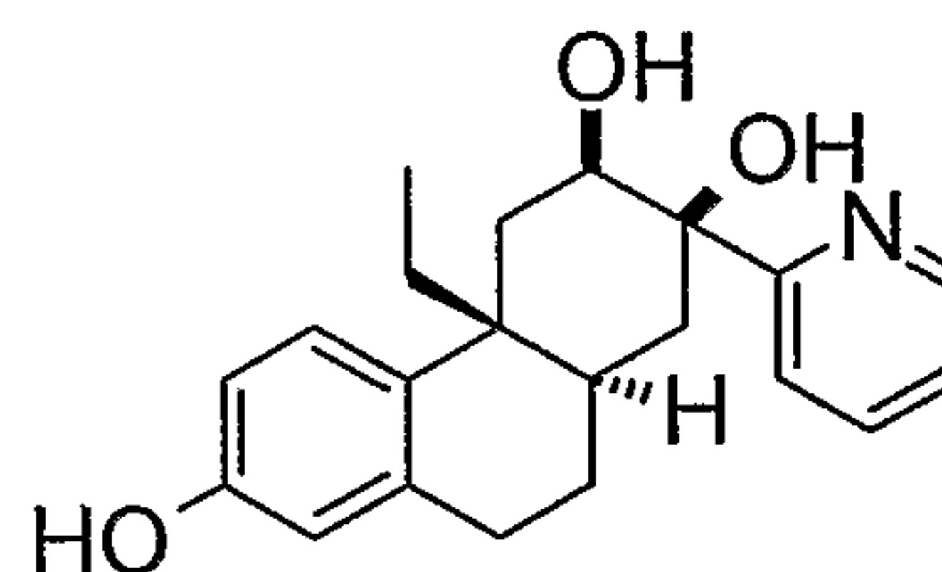
Example 114
