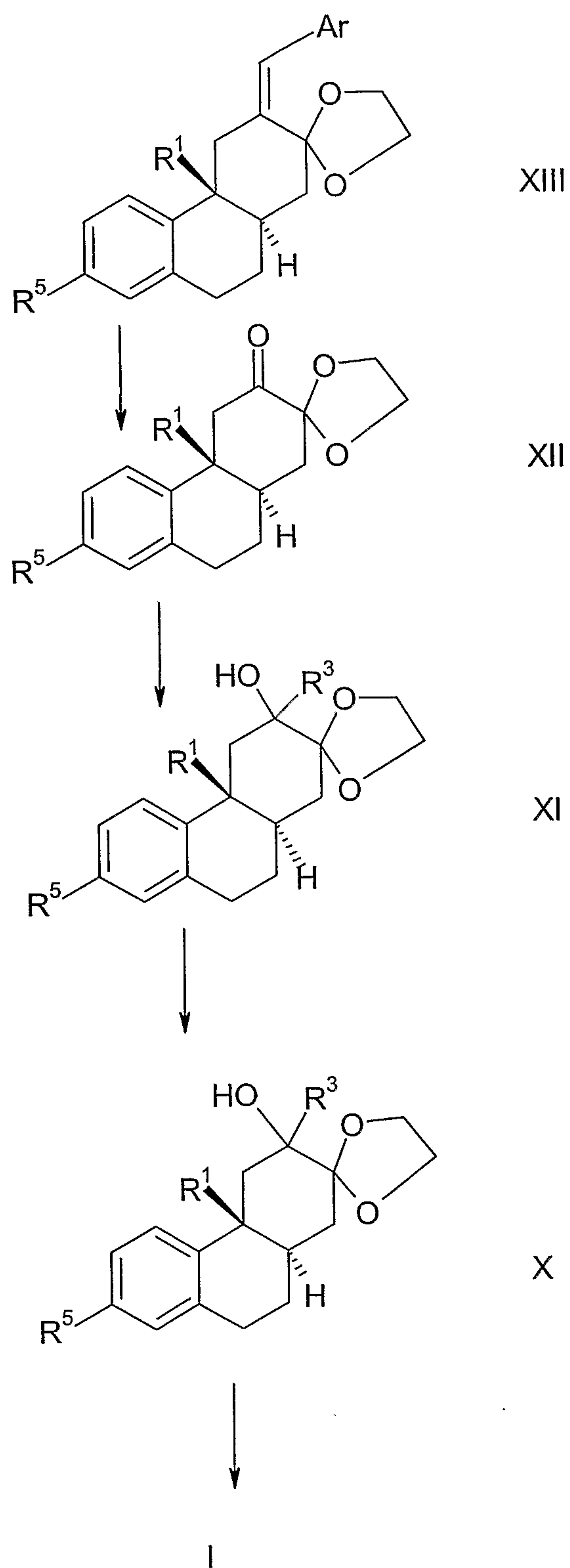
Scheme 4
