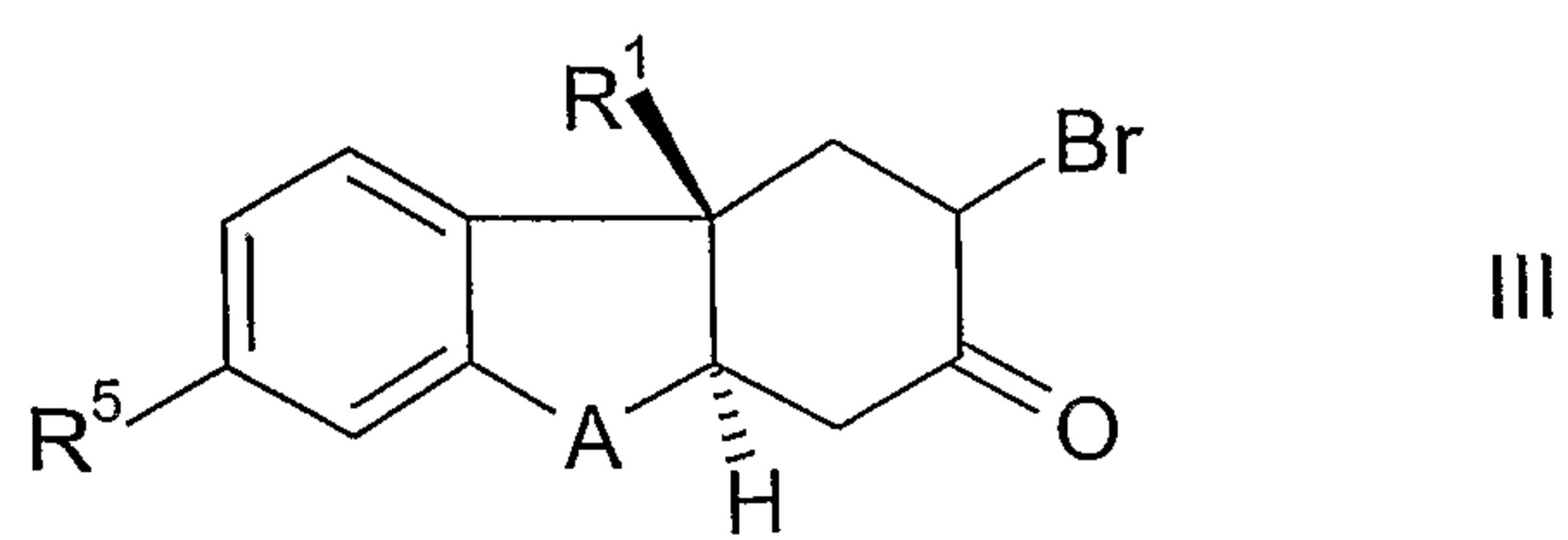
Scheme 5
