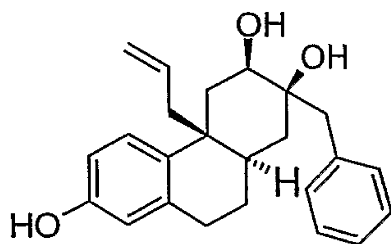
Example 23
