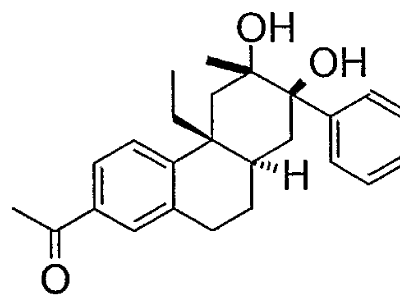
Example 120
