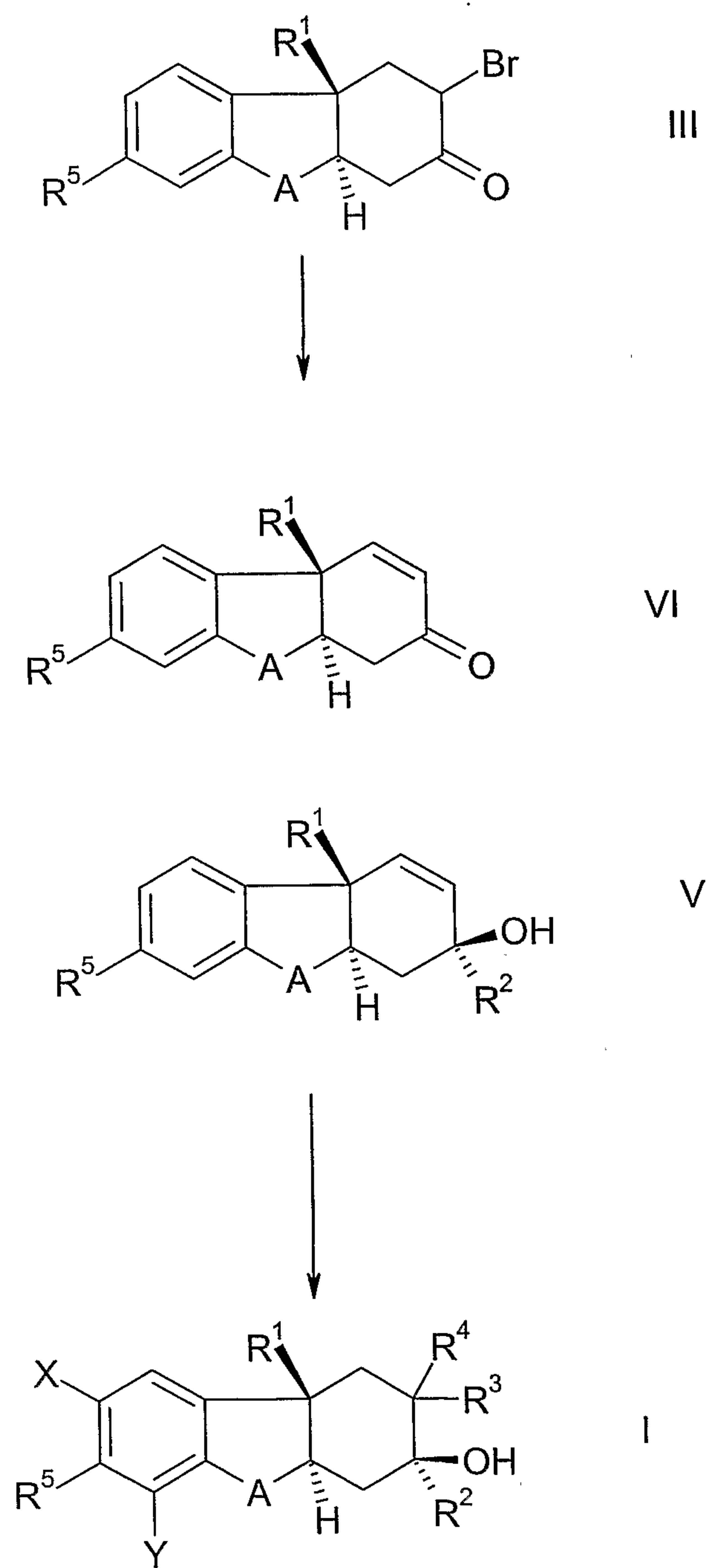
Scheme 2
