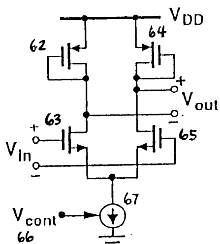
SINGLE DIFFERENTIAL STAGE
