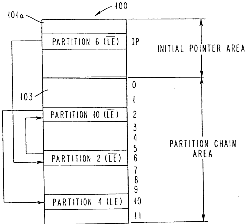
FIG. 16 TRANSMIT LIST STRUCTURE IN BURST PRIORITY RAM
