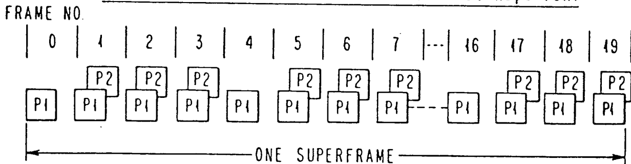
FIG. 10 PORT CHANNELS SENT (ASSUMING NO DAC) FOR 56 Kbps PORT
