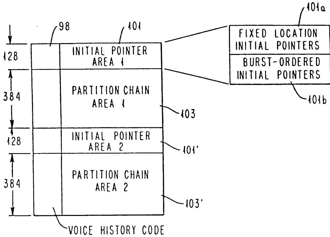
FIG. 15 BURST PRIORITY RAM 100
