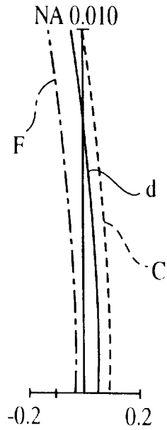
LONGITUDINAL SPHERICAL ABERRATION
