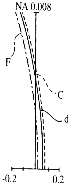
LONGITUDINAL SPHERICAL ABERRATION
