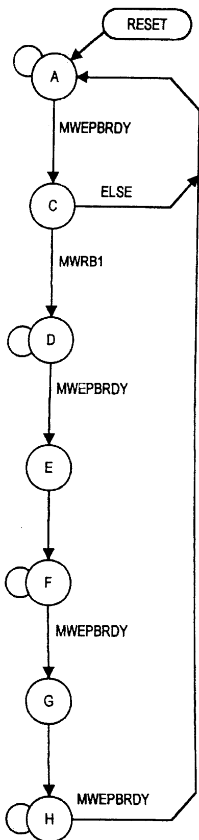
MPMLE STATE MACHINE
