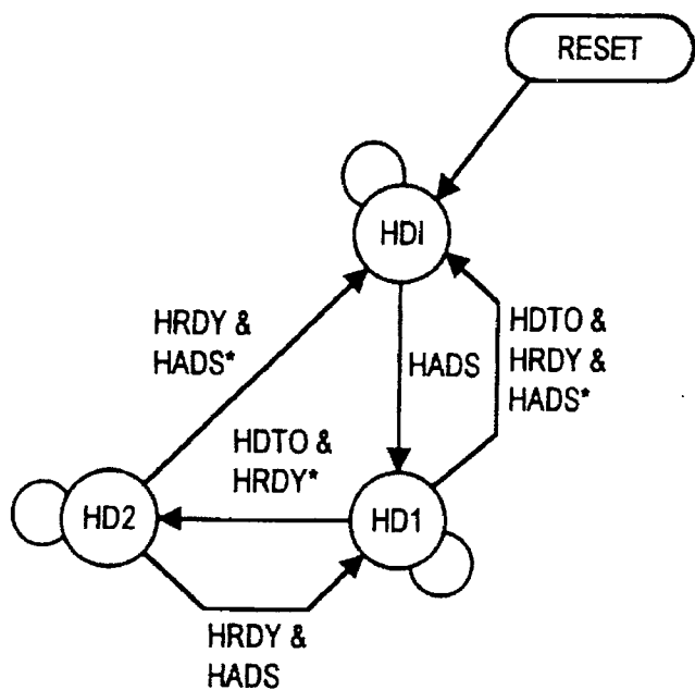
HDAT STATE MACHINE
