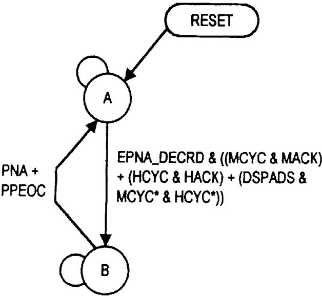
RDPNA STATE MACHINE
