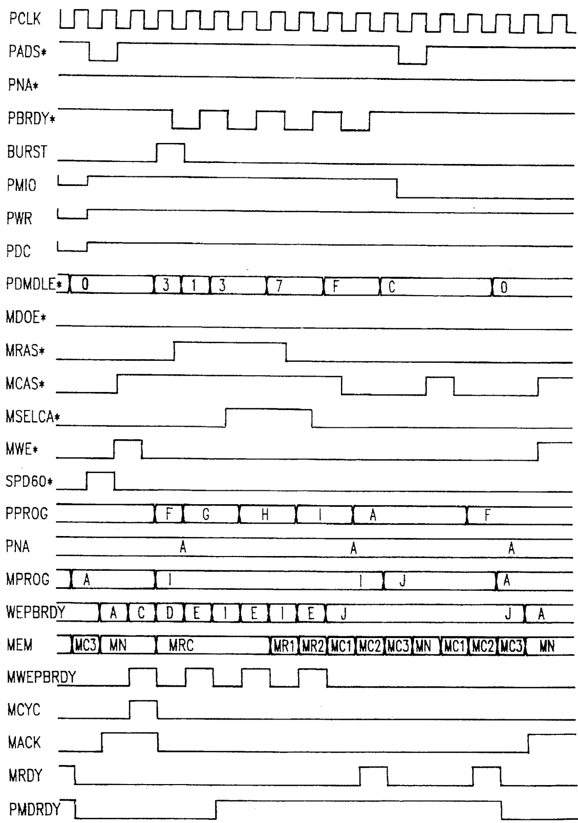
MEMORY WRITE BURST, PAGE MISS, w/60ns MEMORY
