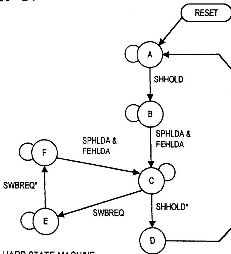
HARB STATE MACHINE
