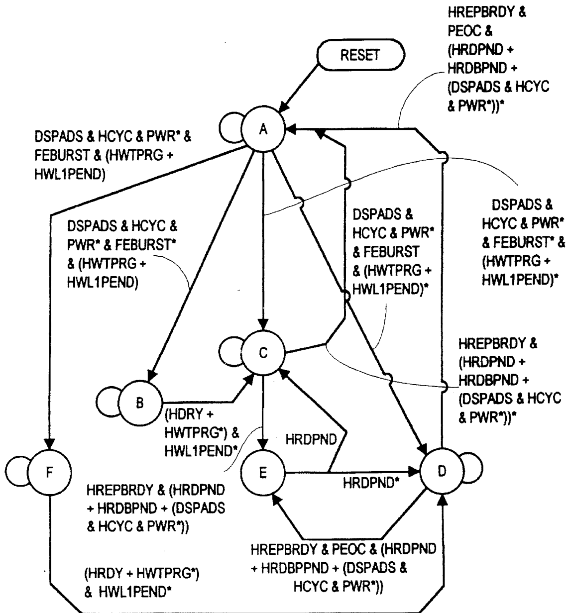
HRD STATE MACHINE
