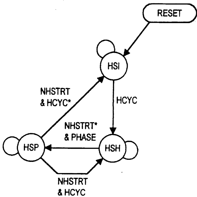
HSYNC STATE MACHINE
