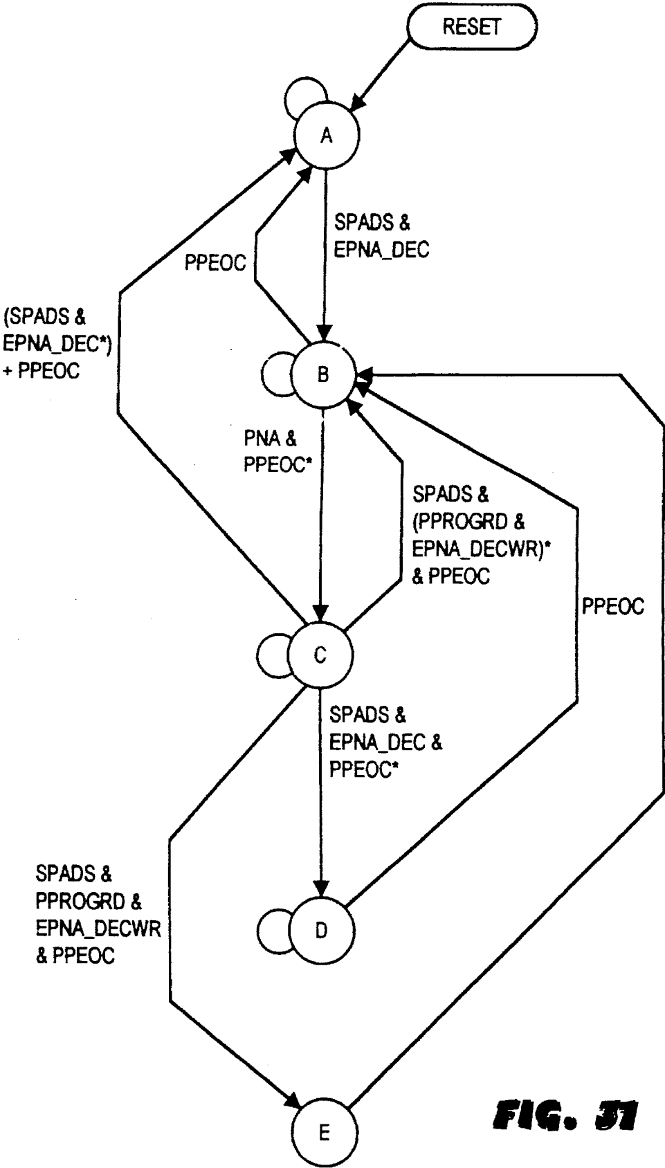
PNA STATE MACHINE
