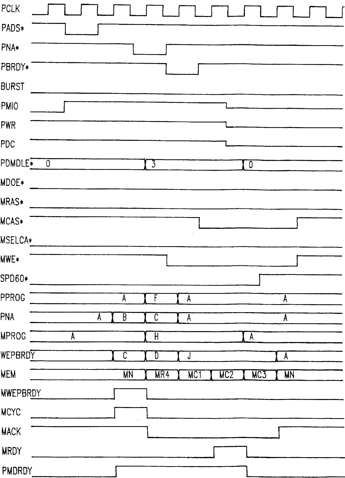
MEMORY WRITE, PAGE HIT, w/60ns MEMORY
