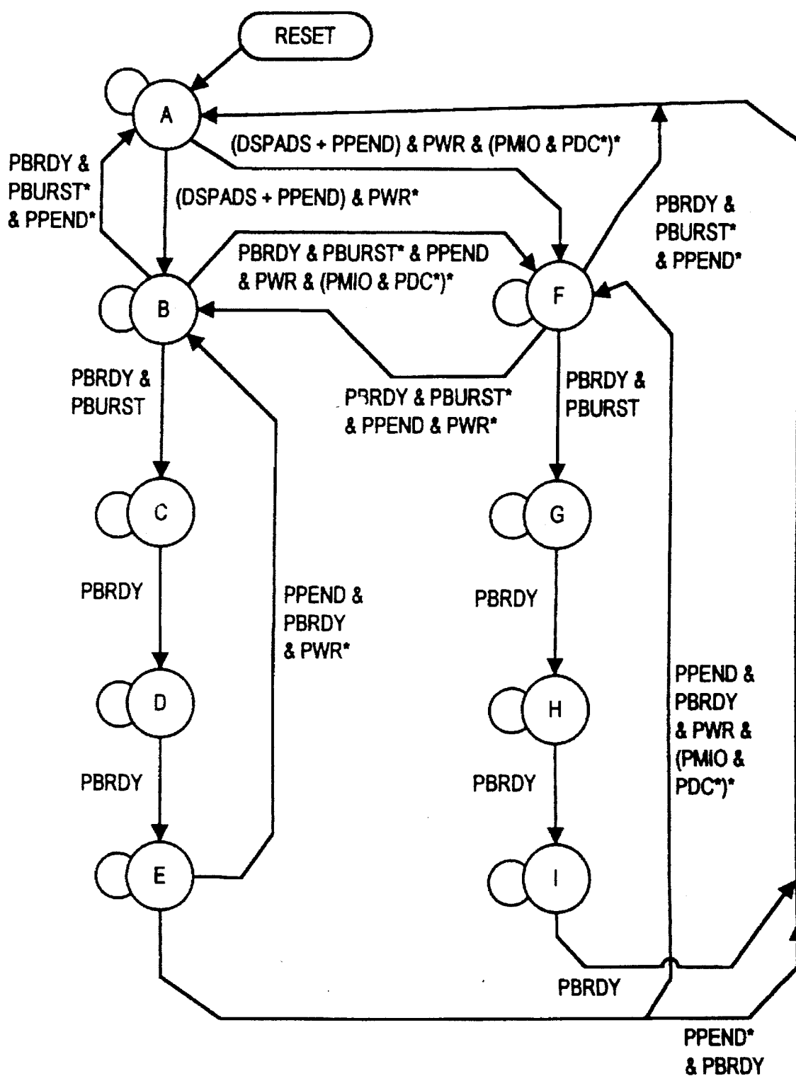
PPROG STATE MACHINE
