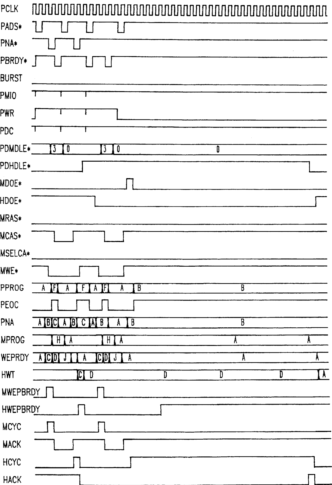
MEMORY WRITE/HOST WRITE, FULLY PIPELINED
