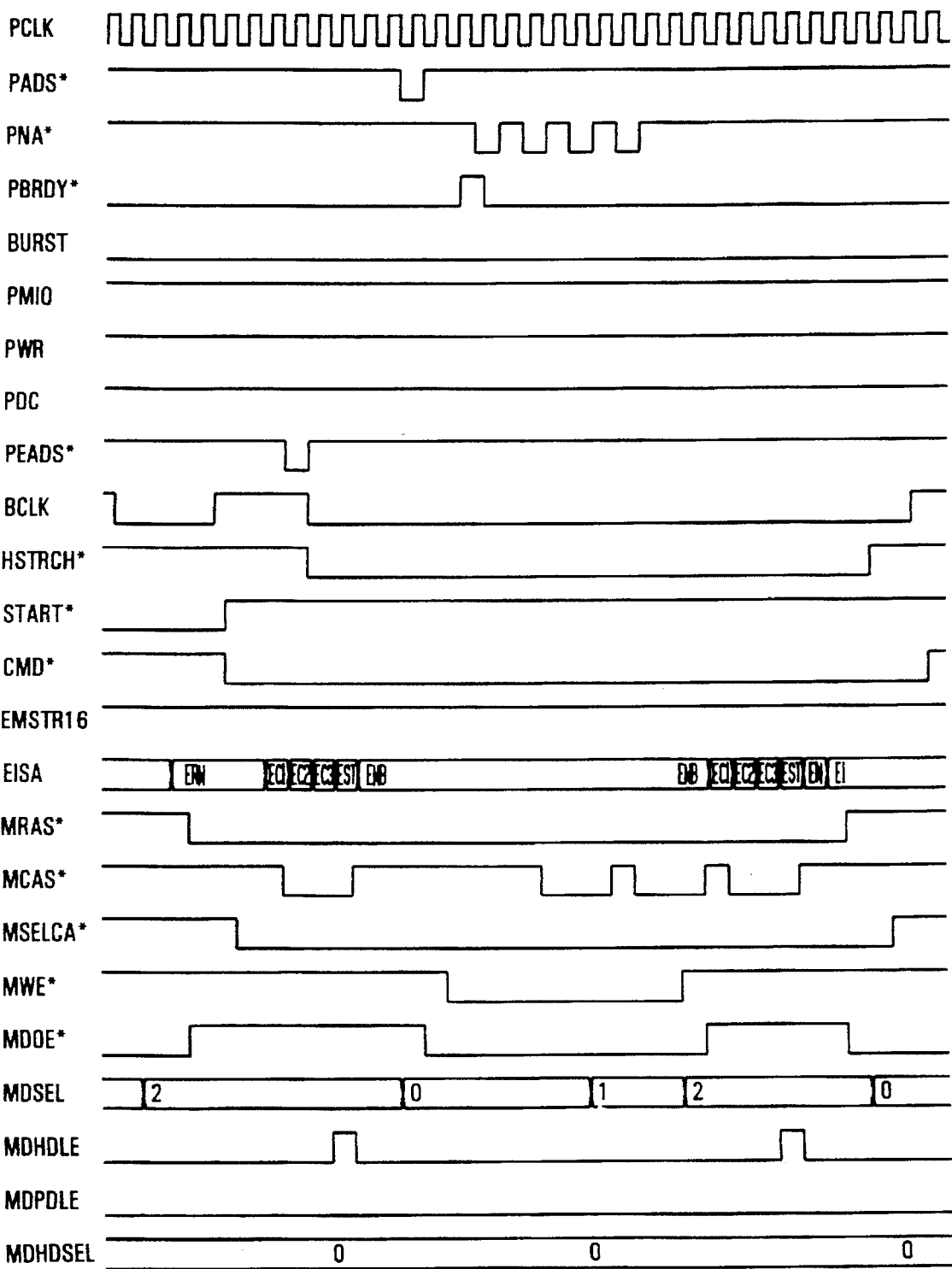
EISA BUS MASTER READ HIT TO MODIFIED
