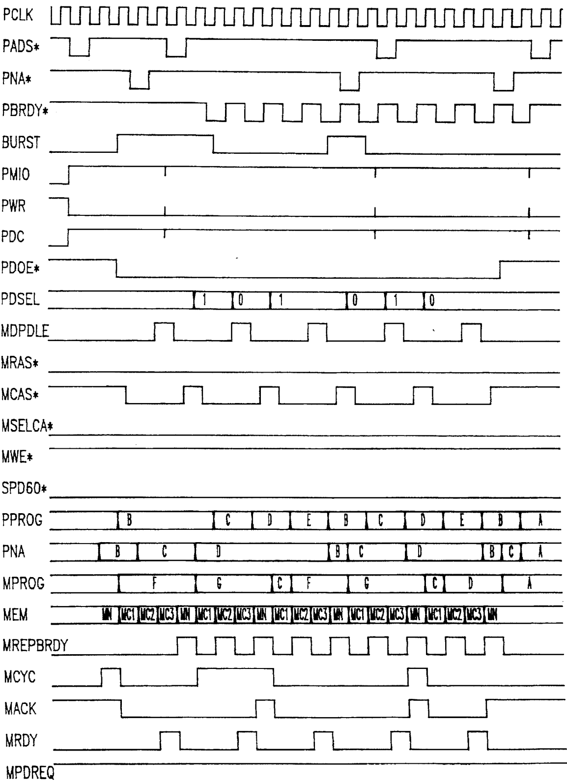
MEMORY READ/MEMORY READ, FULLY PIPELINED
