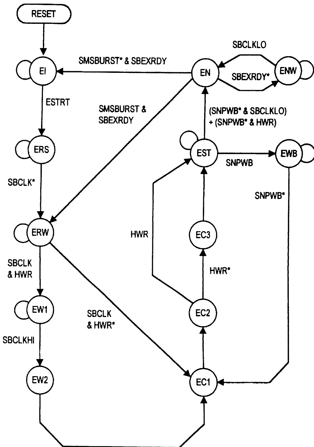
EISA STATE MACHINE
