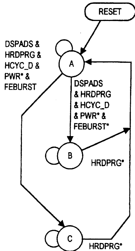
HRDPND STATE MACHINE
