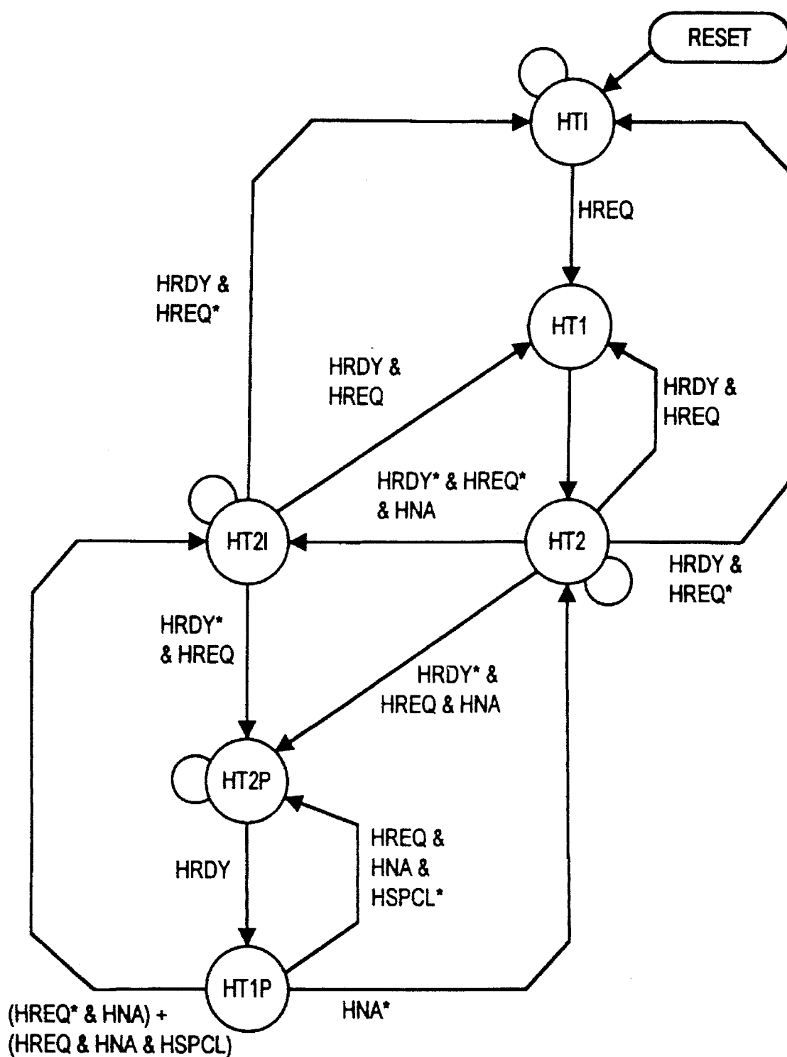
HOST STATE MACHINE
