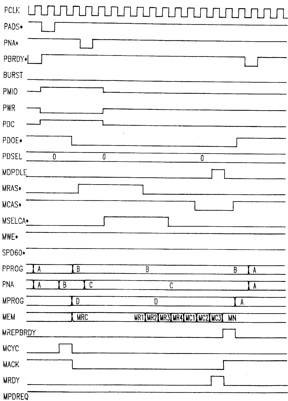
MEMORY READ, PAGE MISS, w/80ns MEMORY
