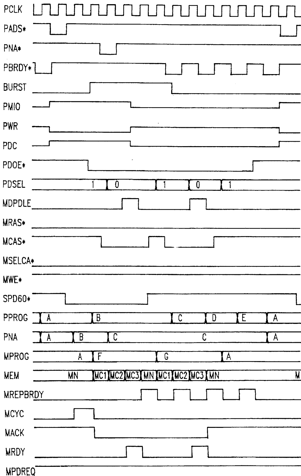
MEMORY READ BURST, PAGE HIT, w/60ns MEMORY
