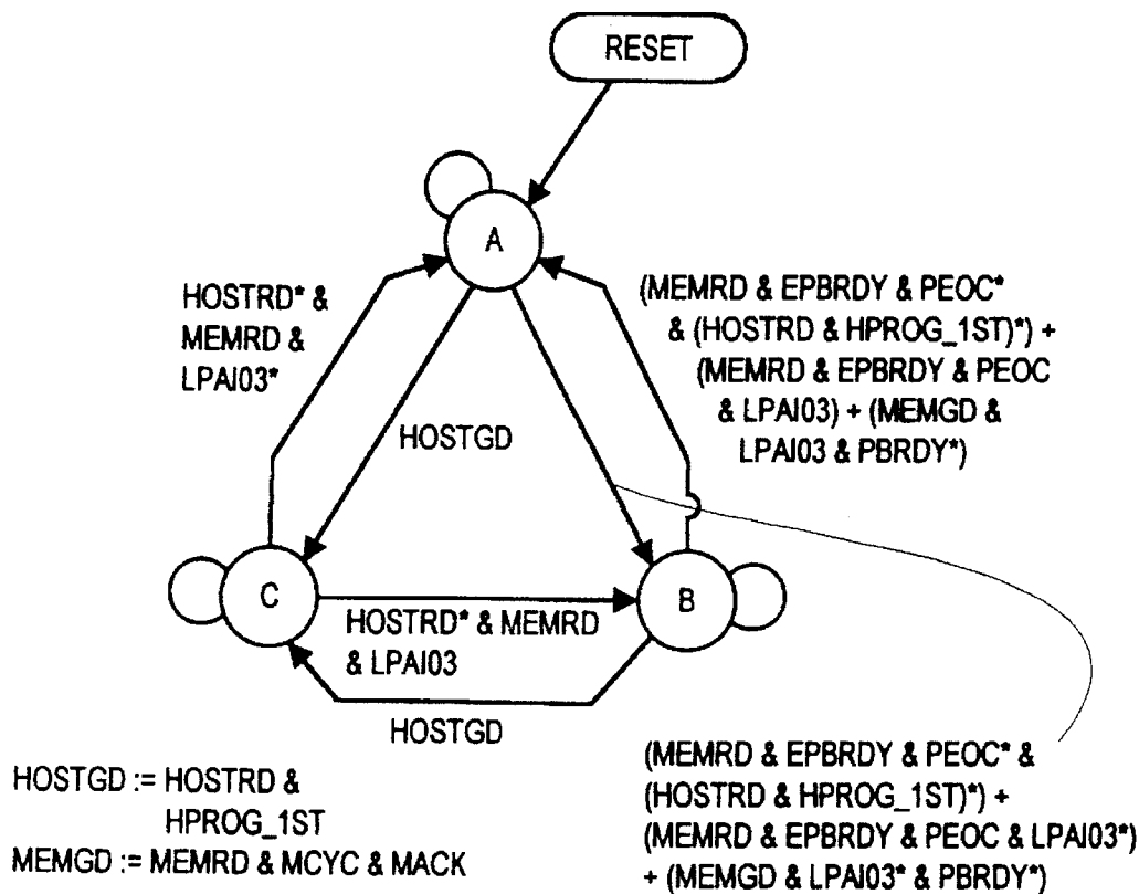
DPSEL STATE MACHINE
