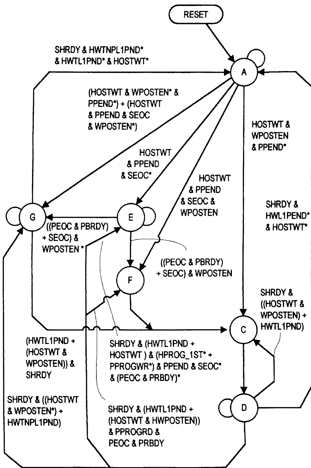
HWT STATE MACHINE
