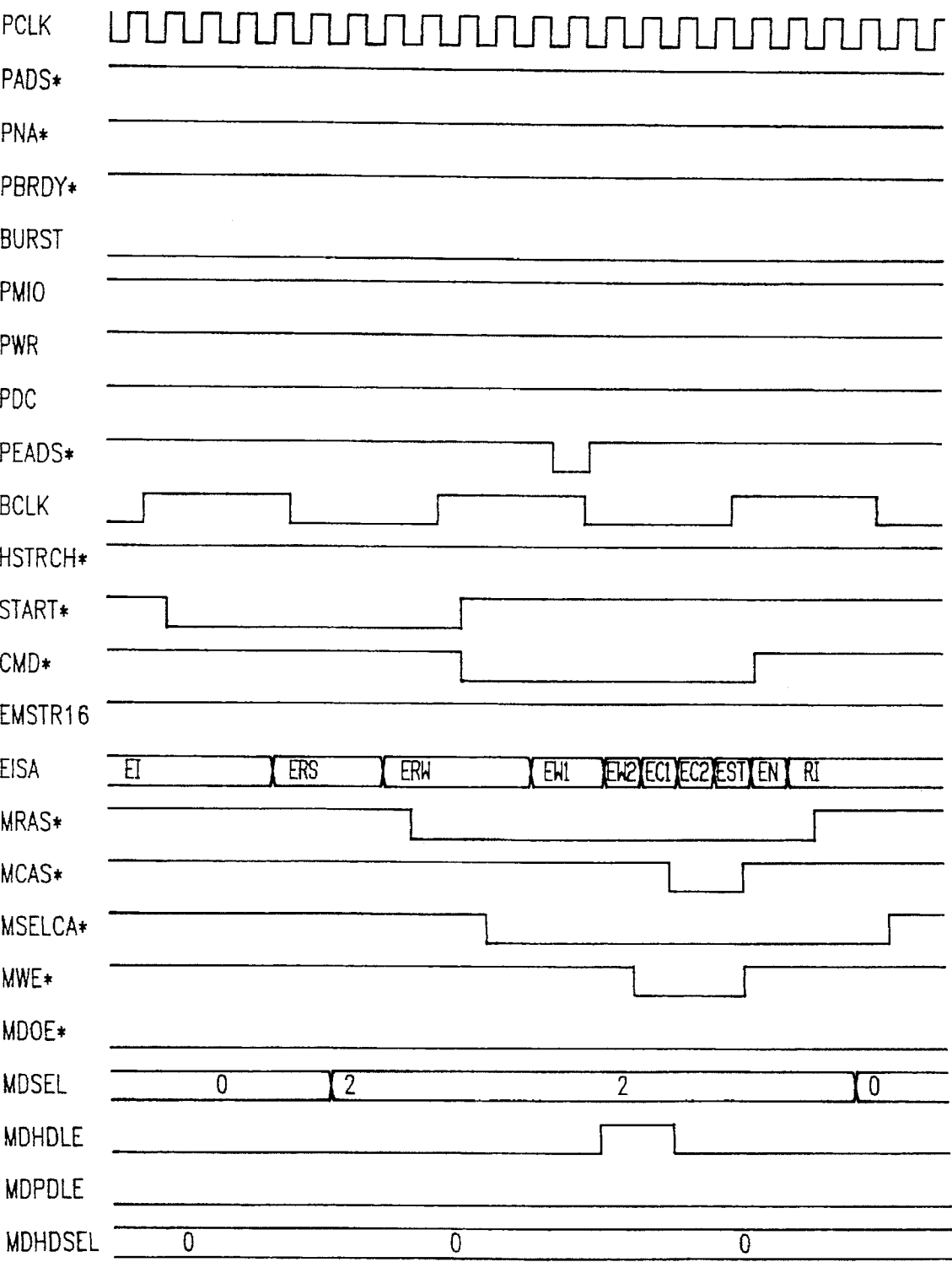
EISA BUS MASTER WRITE CYCLE
