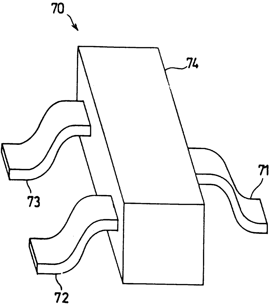
FIG. 22 PRIOR ART
