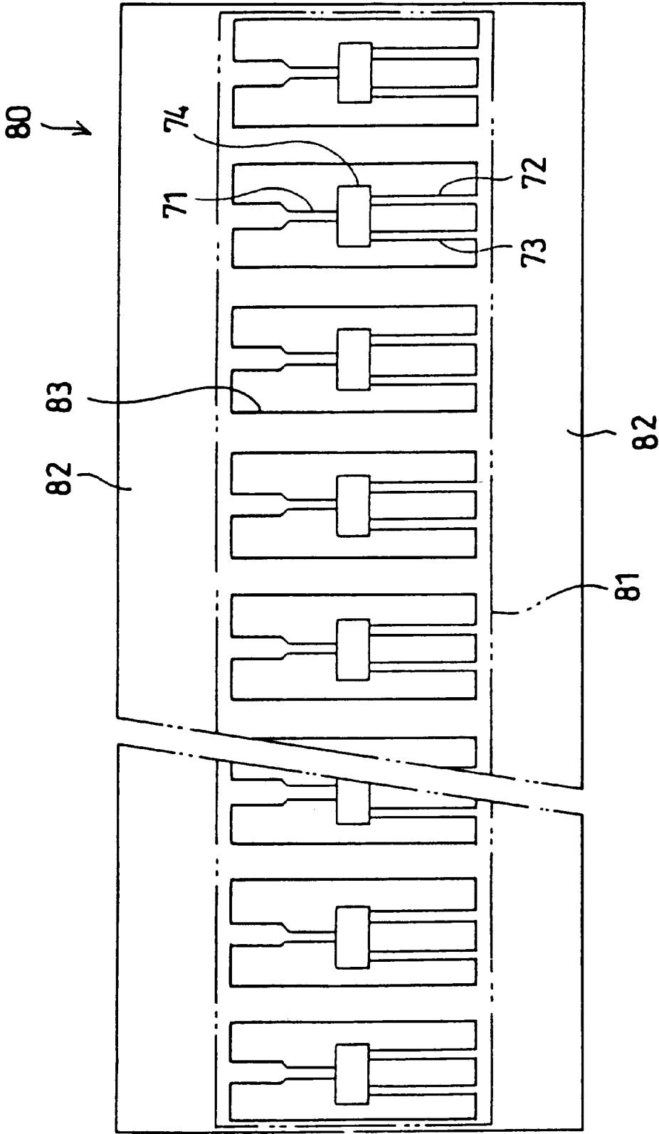
FIG. 24 PRIOR ART
