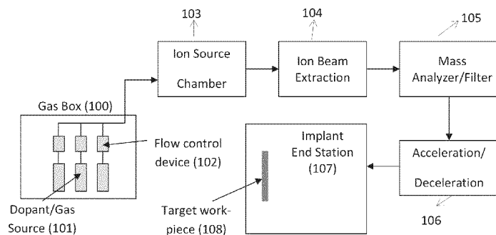
Schematic of beamline ion implant system
