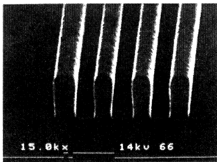
FIG. 18 PRIOR ART
