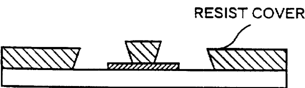
FIG. 5B RESIST PATTERNING
