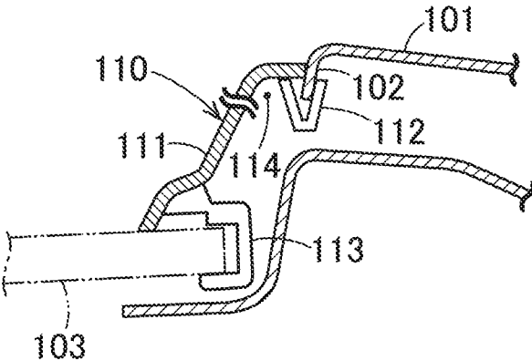
FIG. 10 (PRIOR ART)
