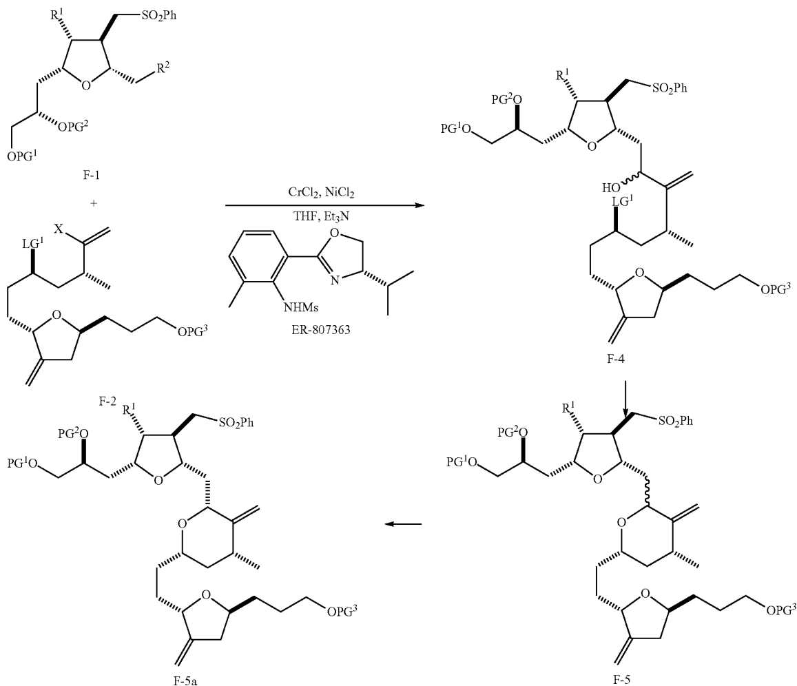
Scheme VIII
