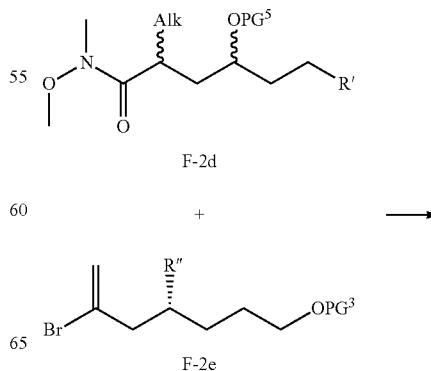
Scheme A
