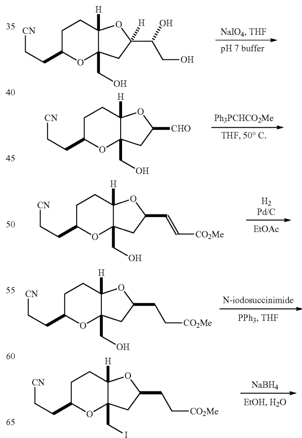
Scheme VI-b
