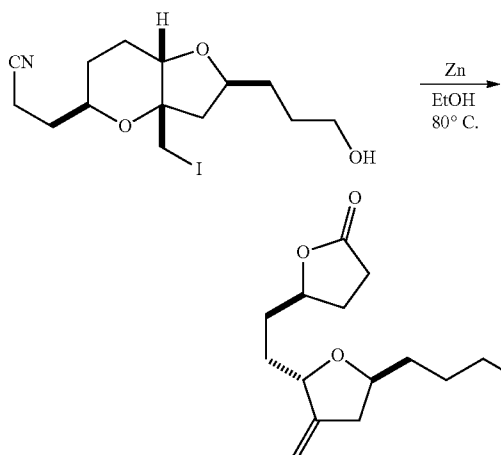
C.14-C.26 lactone
