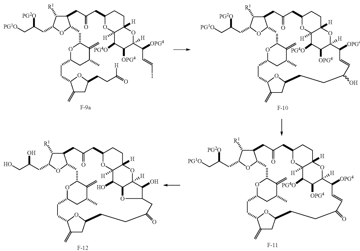
Scheme X
