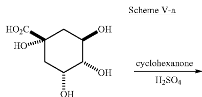
D-quinic acid
