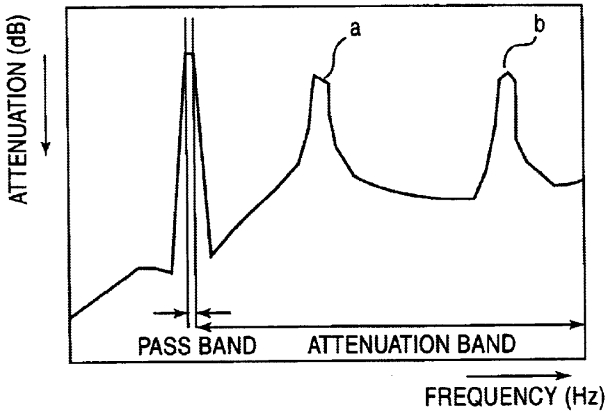
FIG. 8 PRIOR ART
