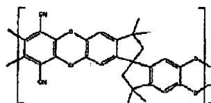
Polydioxane A (1)
