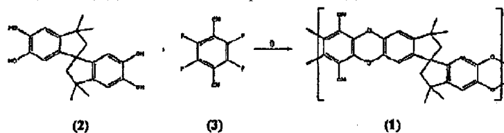
Reaction scheme A: synthesis of polydioxane A (1); i) K_2CO_3 , DMF, 50°C
