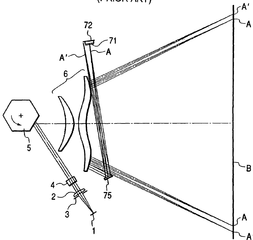
FIG. 6 (PRIOR ART)
