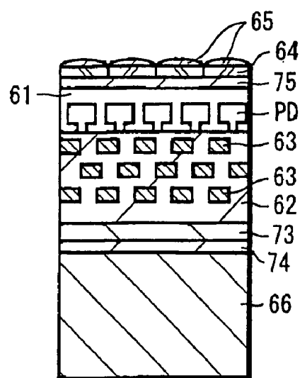
FIG. 3E (RELATED ART)
