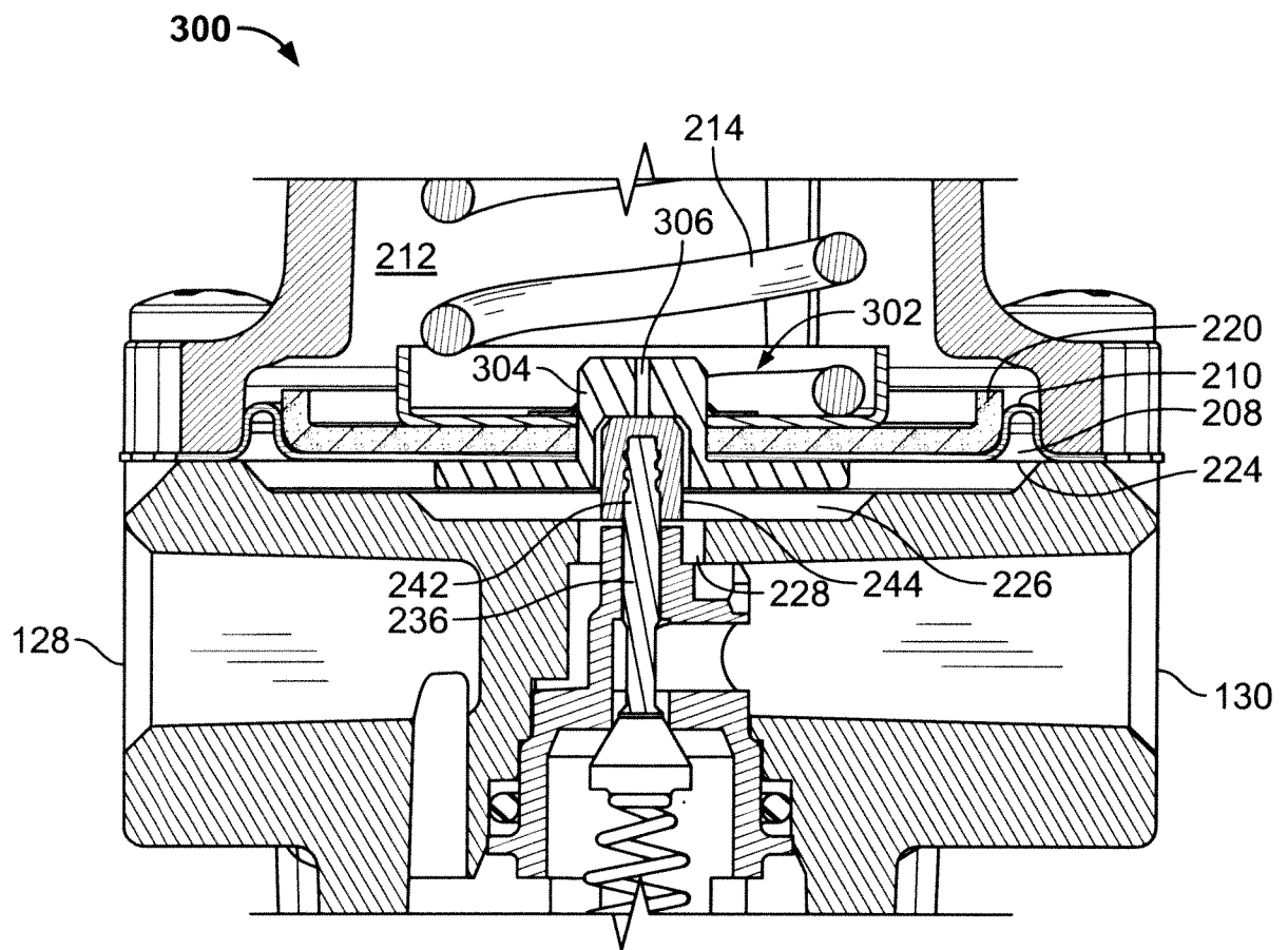
FIG. 3 (Prior Art)
