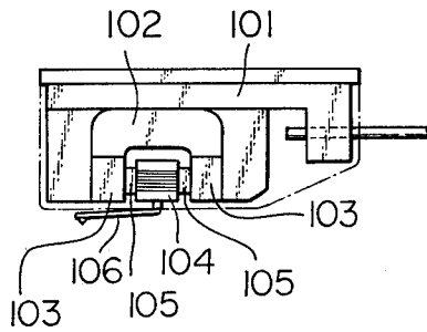
Fig. 1 (PRIOR ART)
