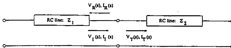
Figure 2: Connection of two RC lines showing incident and transmitted components at the junction.
