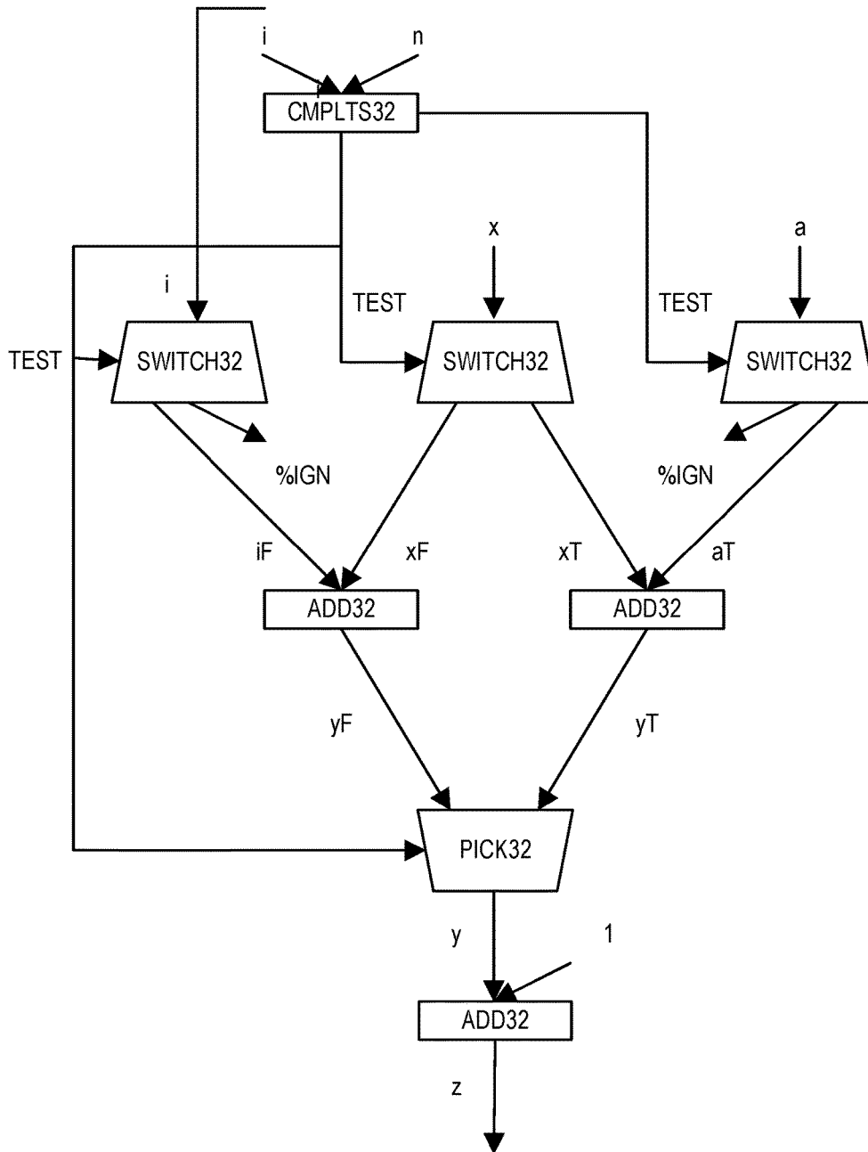
DATAFLOW GRAPH 1806
