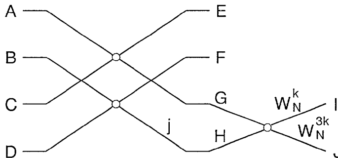
Basic Split Radix Butterfly
