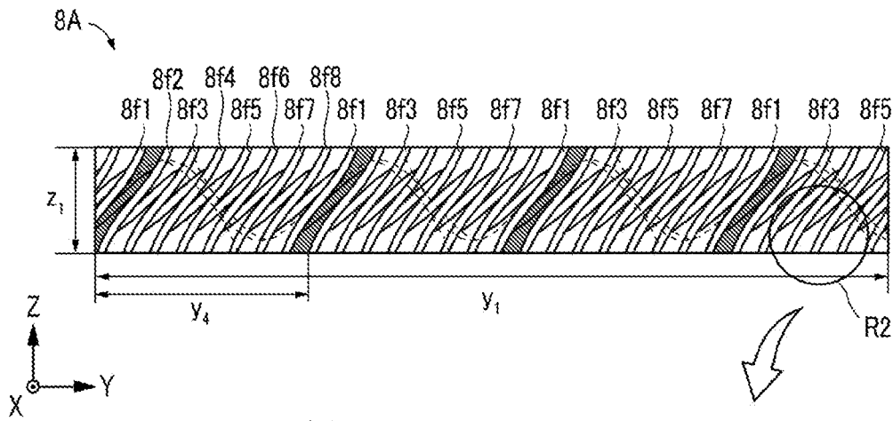
FIG. 7(a) SIDE SURFACE VIEW
