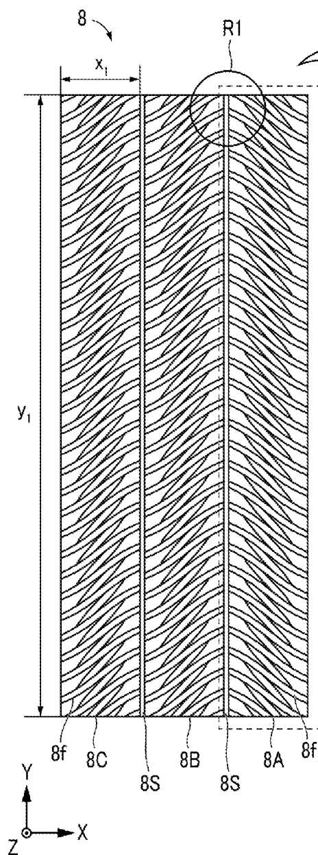
FIG. 3(a) UPPER SURFACE VIEW
