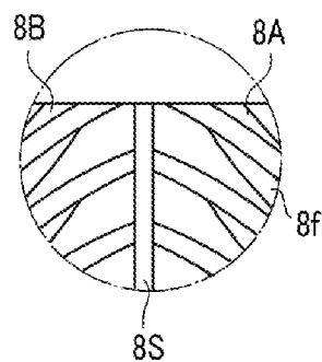
FIG. 3(b) ENLARGED VIEW (REGION R1)
