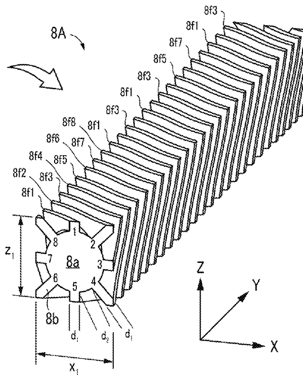
FIG. 3(c) PERSPECTIVE VIEW (COOLING FIN 8A)
