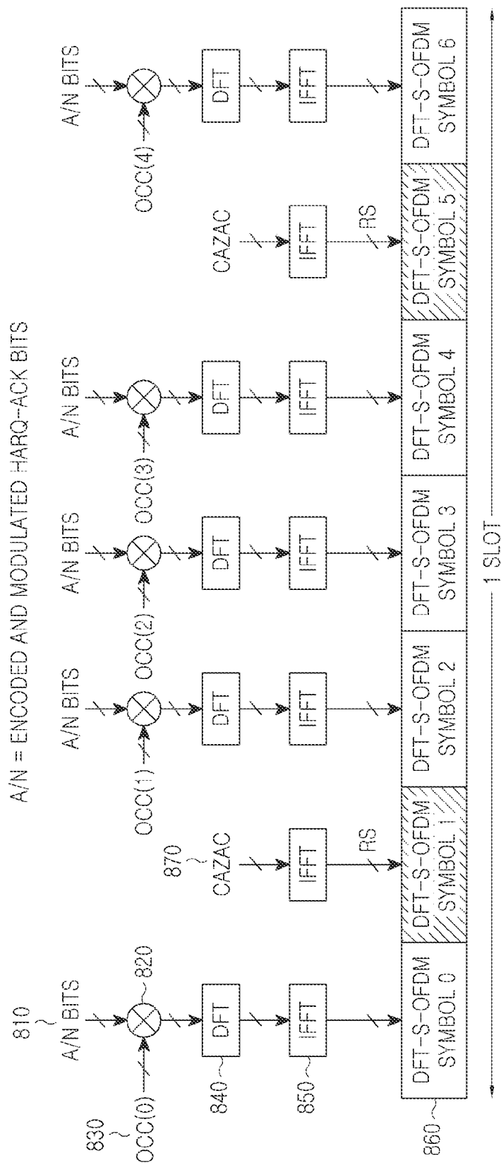
FIG. 8 (PRIOR ART)
