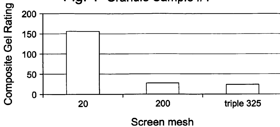
Fig. 1 Granule Sample #1
