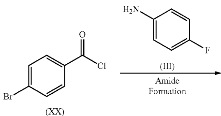
Scheme 2: Preparation of Compound (I) by Route 4.
