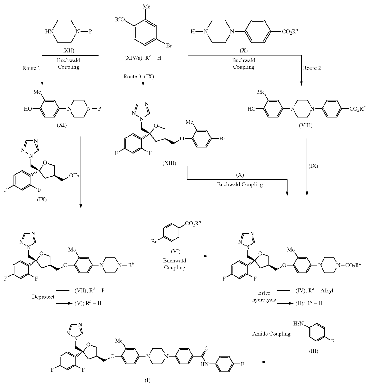
Scheme 1: Preparation of Compound (I) by Routes 1-3.
