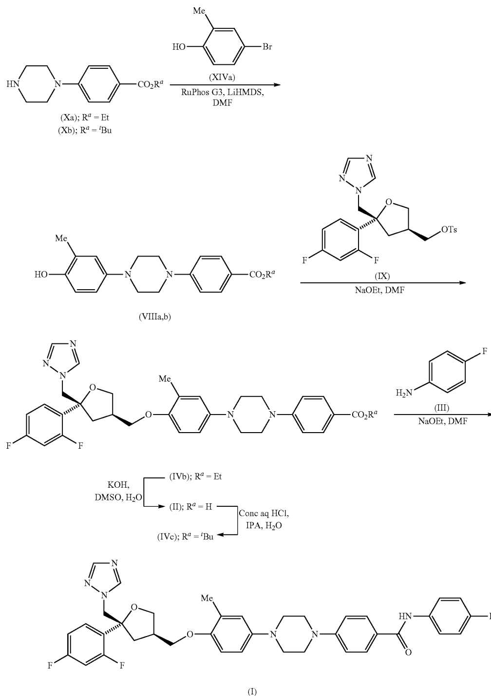
Scheme 3: Scale-Up of the Synthesis of Compound (I)
