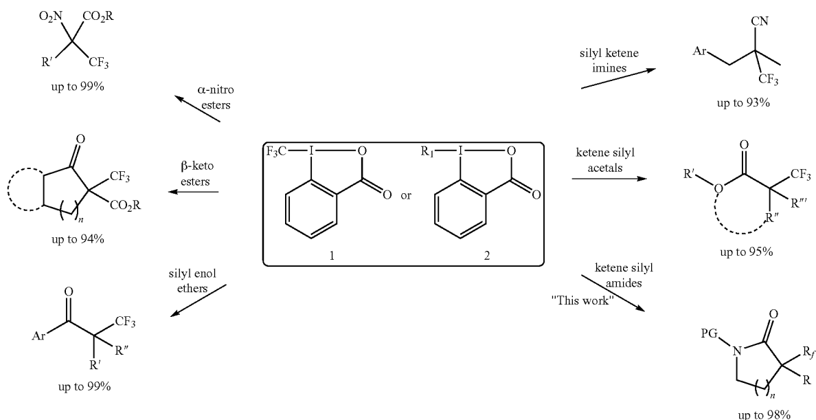
Scheme 5 Application of hypervalent iodine(III)-R f reagents 1 and 2 in the formation of a quaternary carbon center.
