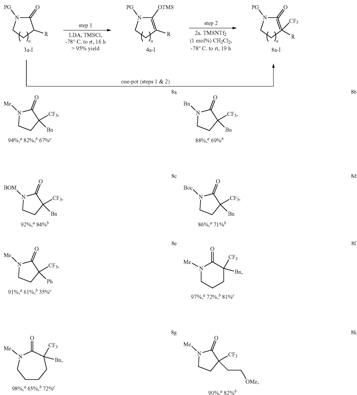
Scheme 6 \alpha -Trifluoromethylation of KSAs and direct, one-pot \alpha -trifluoromethylation of carbonyl compounds: lactam scope.
