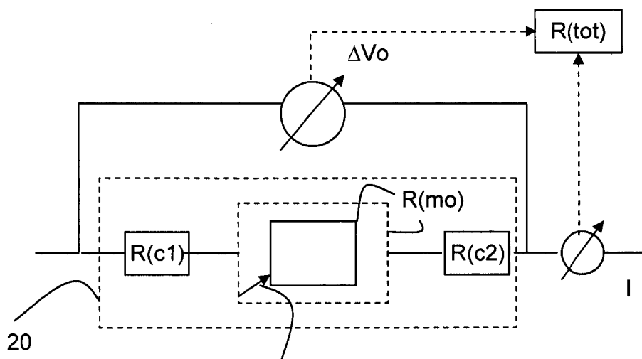
FIG. 2 Reducing sensor dimensions
