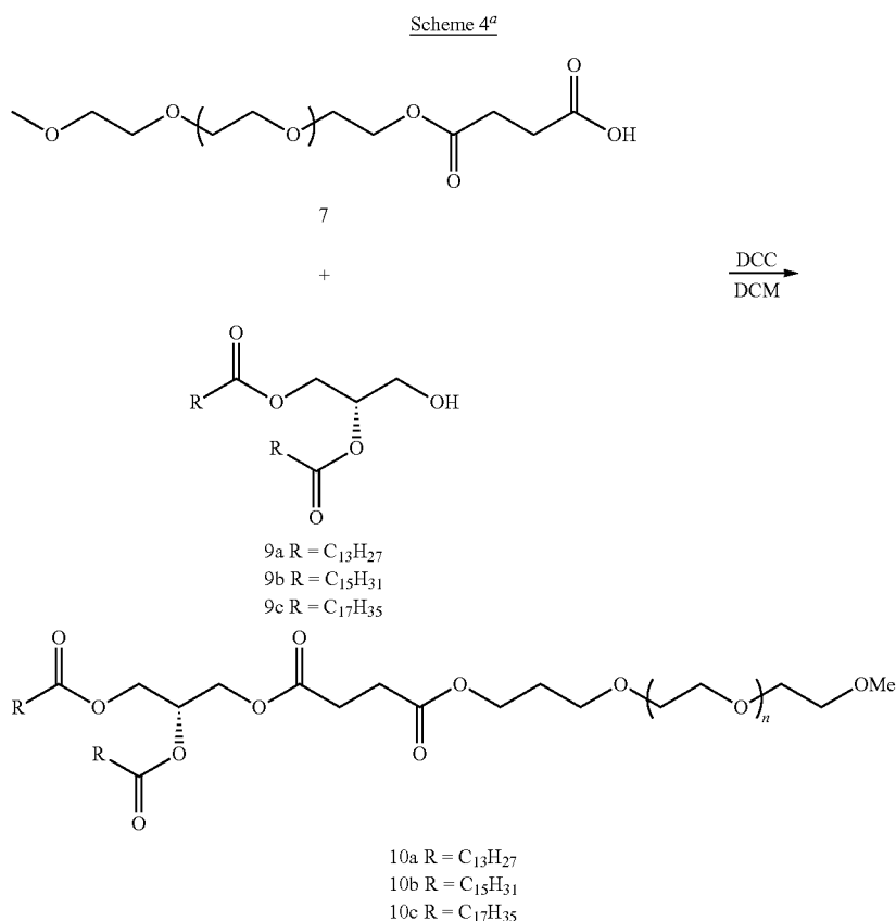
a Scheme 4: mPEG2000-1,2-Di-O-acyl-sn-3-succinylglyceride
