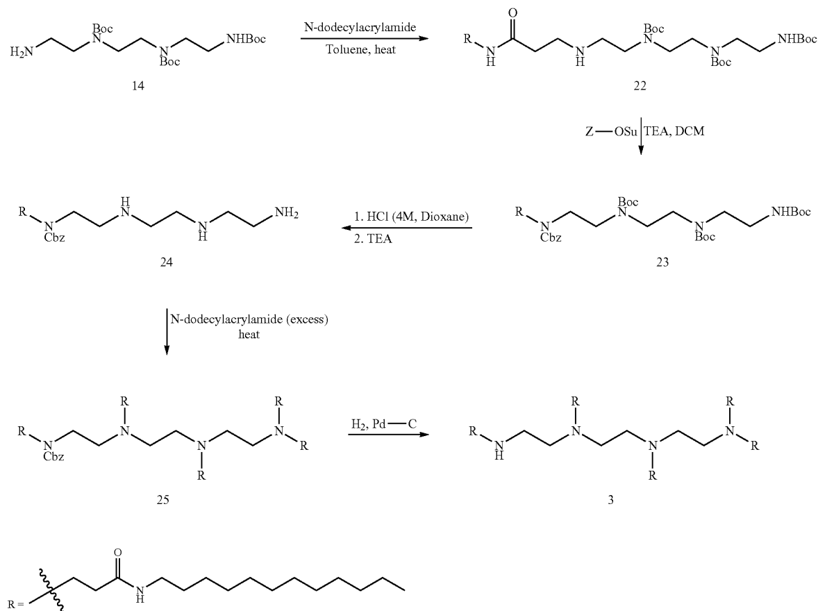
Scheme 12
