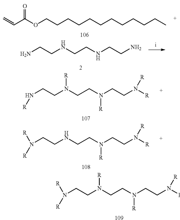
Scheme 28 a
