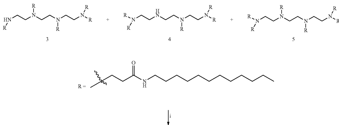
Scheme 19 a
