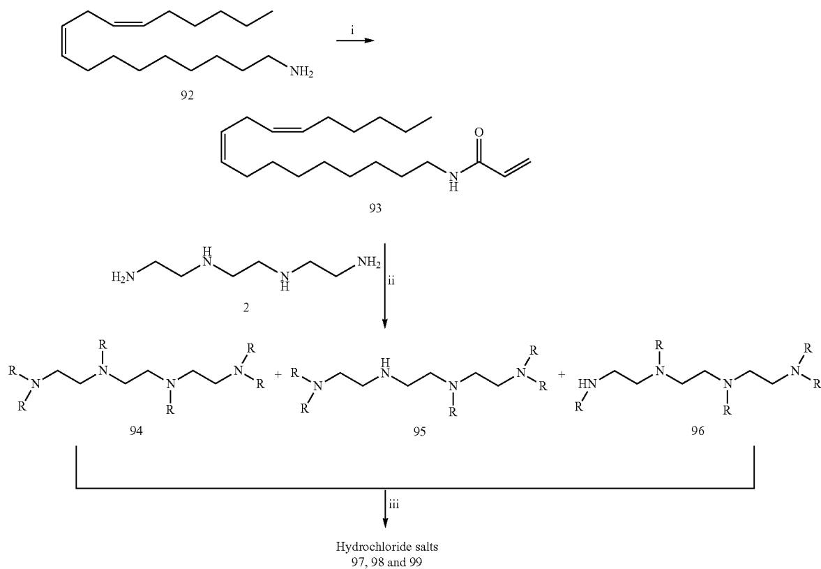
Scheme 26 a
