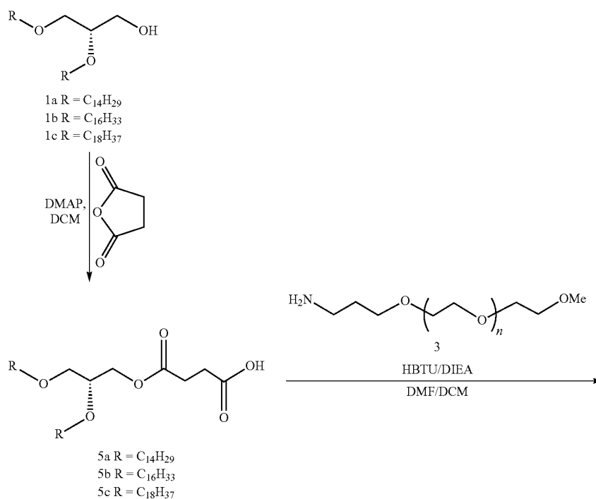
Scheme 2 a
