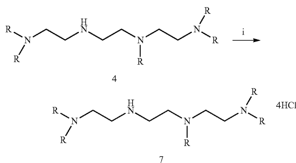
Scheme 6 a
