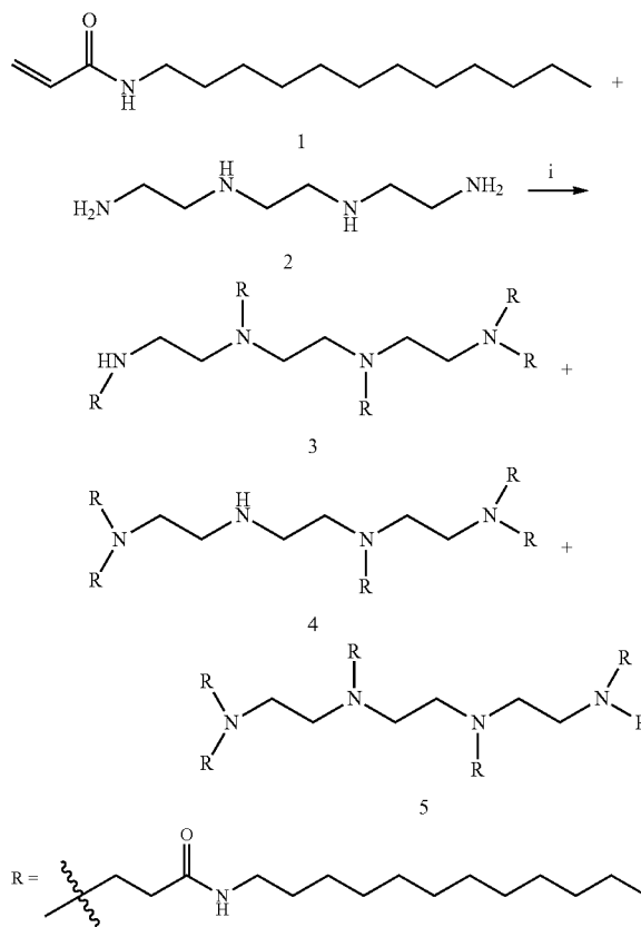
Scheme 3 a
