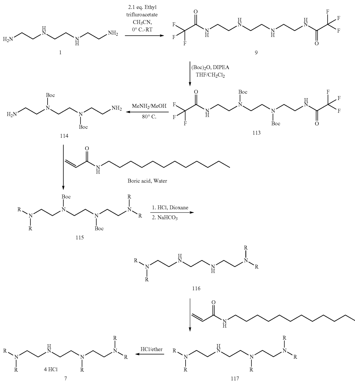
Scheme 31 a
