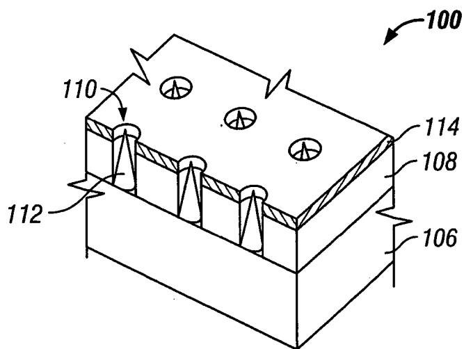
FIG. 3 (Prior Art)
