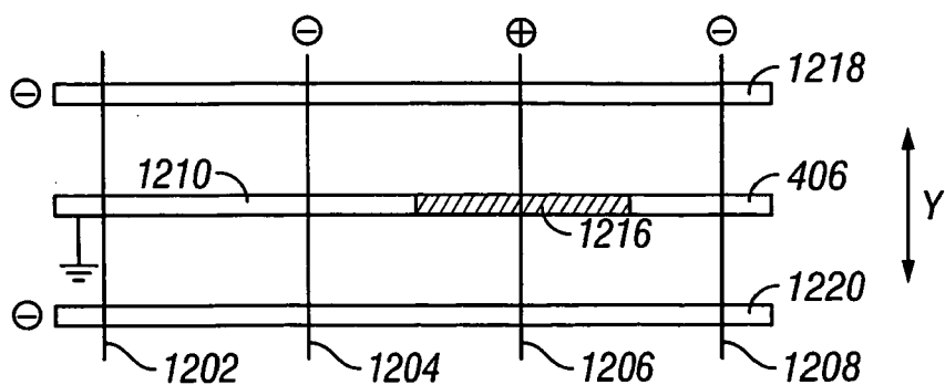
FIG. 12D
