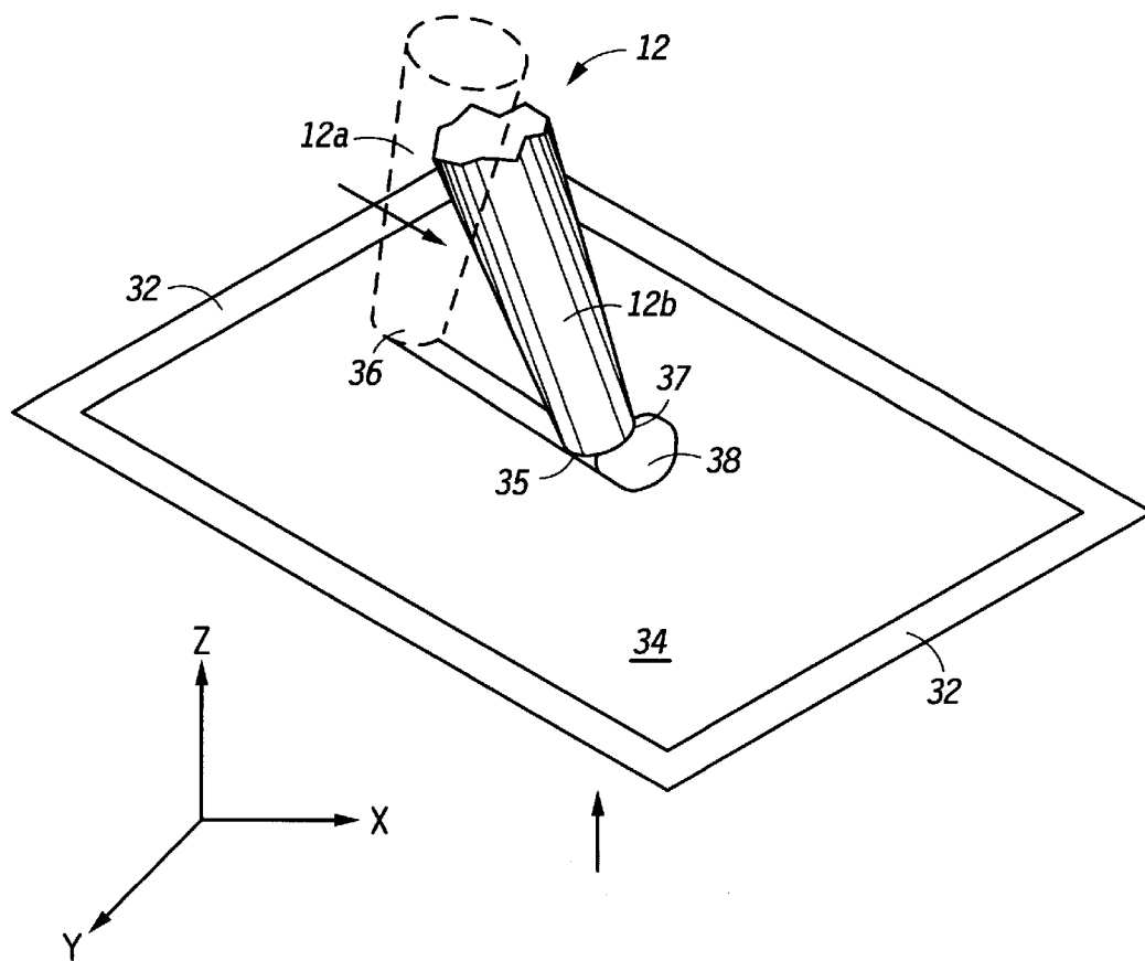
FIG. 2 -PRIOR ART-
