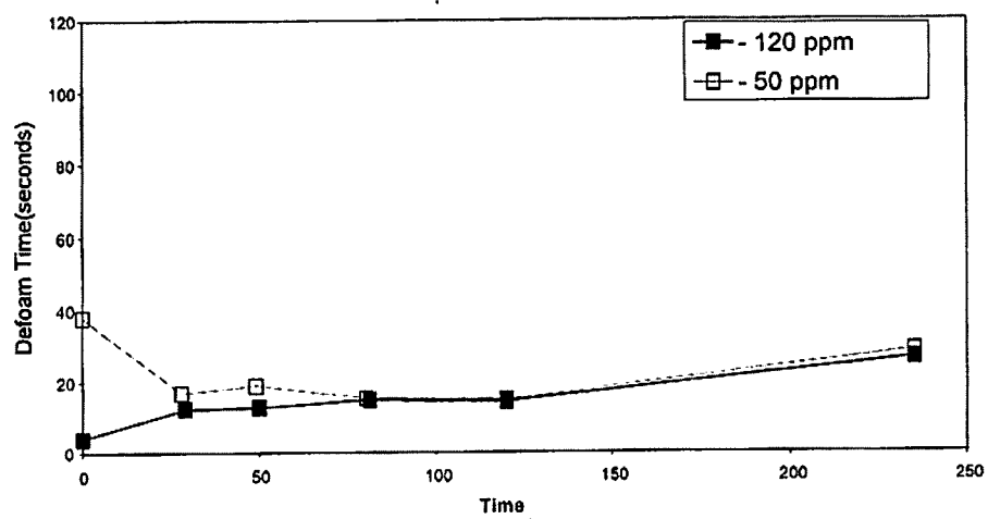
Figure 2: Long Term Foam Control With Antifoam A (10 min Defoam Time)
