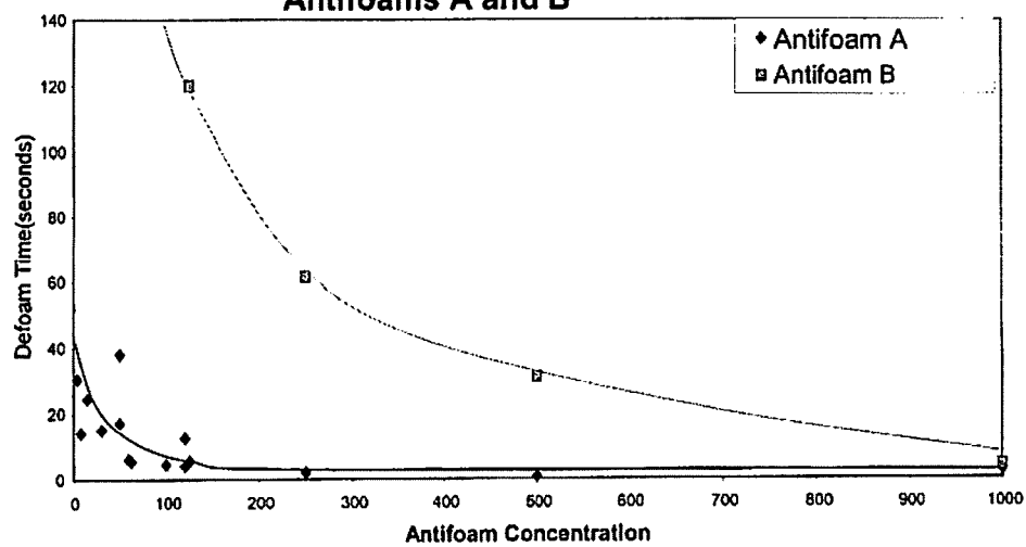
Figure 1: Defoam Rate vs Concentration for Antifoams A and B
