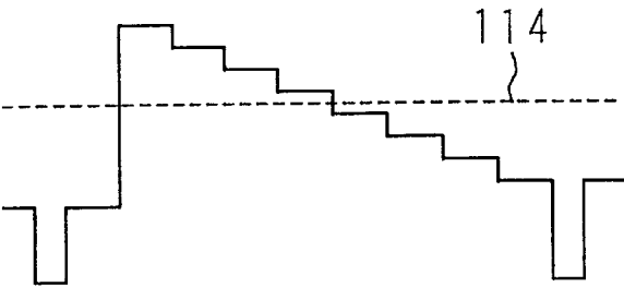
Fig. 29A LUMINANCE SIGNAL Y
