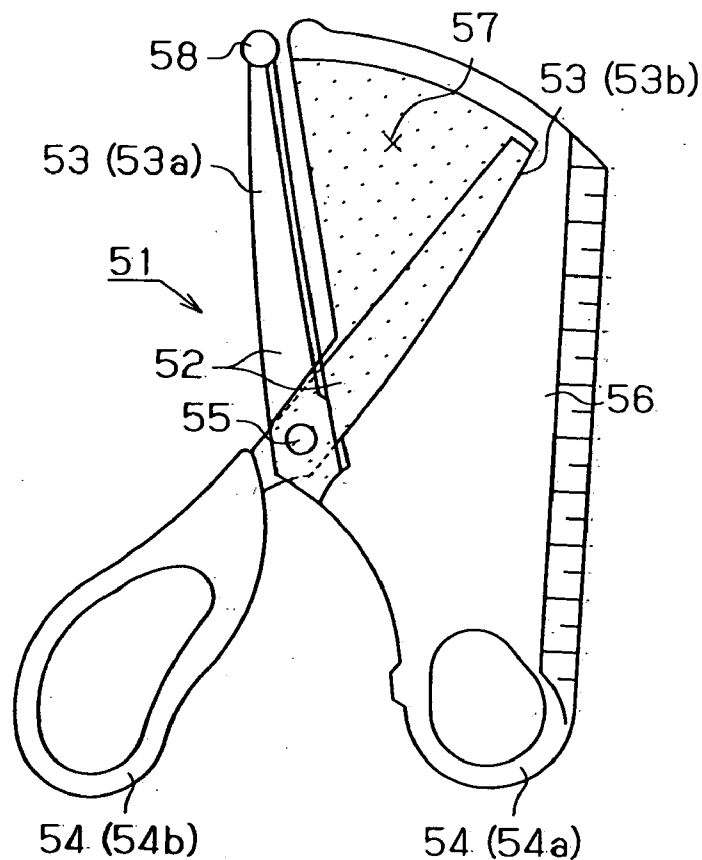
Fig. 9 (Prior Art)
