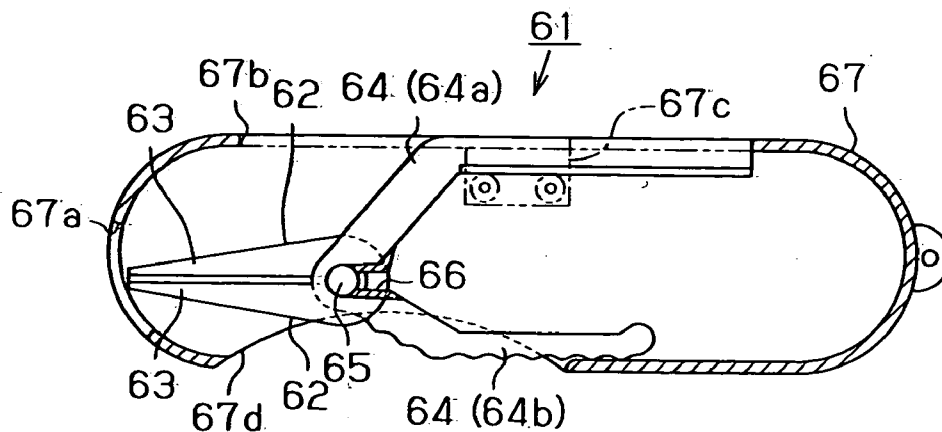
Fig. 10 (Prior Art)
