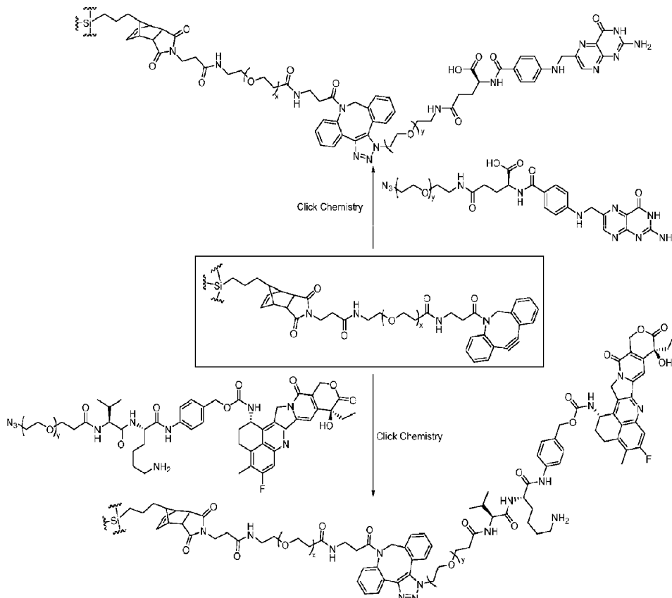
Scheme 7. An exemplary method of functionalizing a nanoparticle with folic acid moieties and exatecan-linker moieties.
