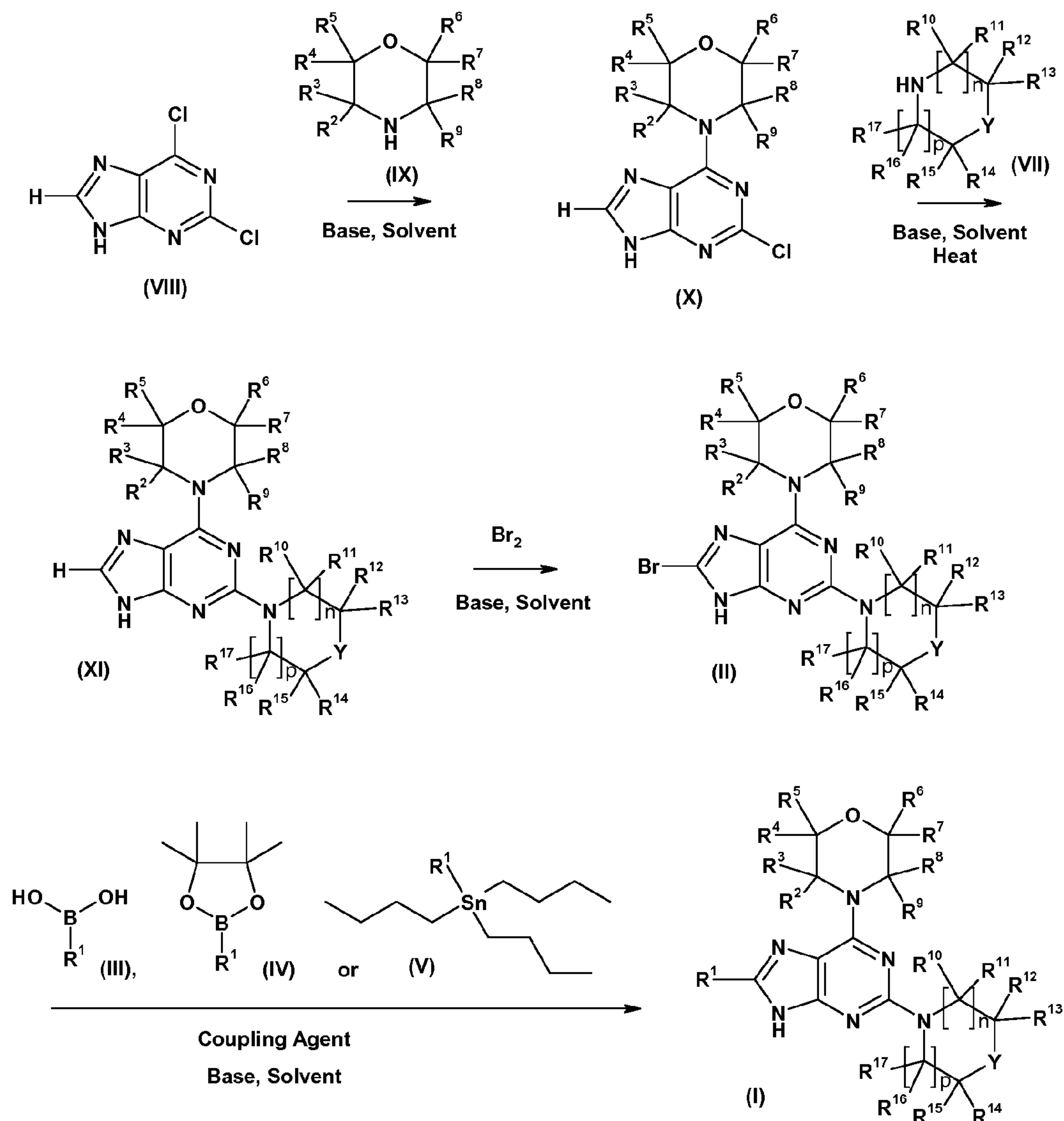
Scheme 1. General Procedure 1 for synthesis of purine compounds
