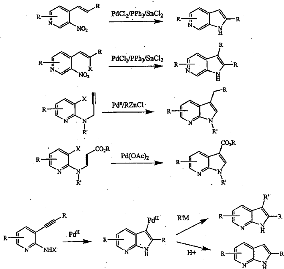
Scheme U: Photochemical
