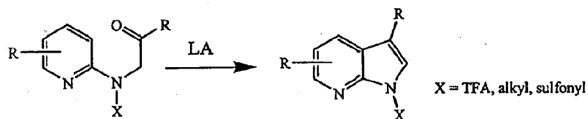
Scheme V: Acid Catalyzed Cyclization
